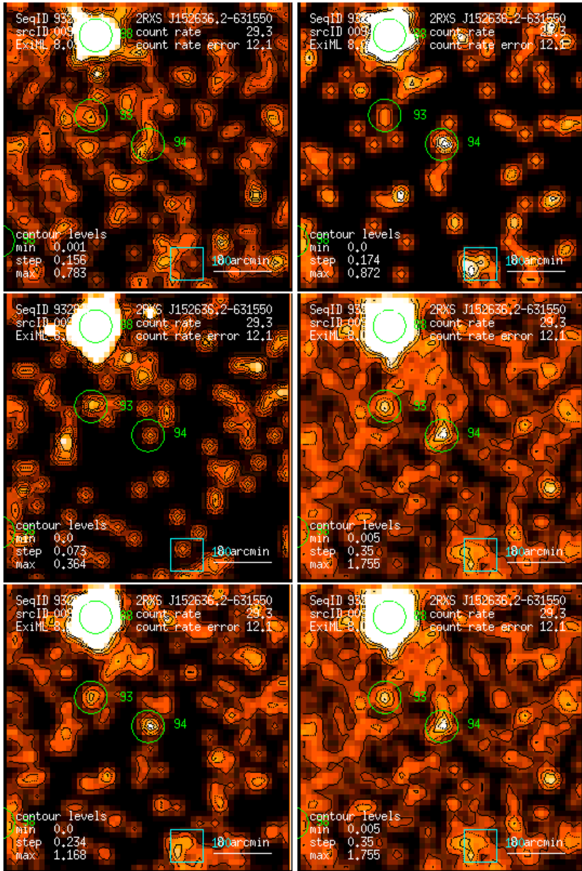
Figure 94: RASS 932822: detection 0094: band rate images, Gaussian filter: (1) PSPC channels 11 – 41, (2) 52 – 90, (3) 91 – 201, (4) 11 – 235, (5) 52 – 201, (6) 11 – 201. Broad band rates in counts/ks. Band rate contour levels in counts/ks/arcmin 2 .
