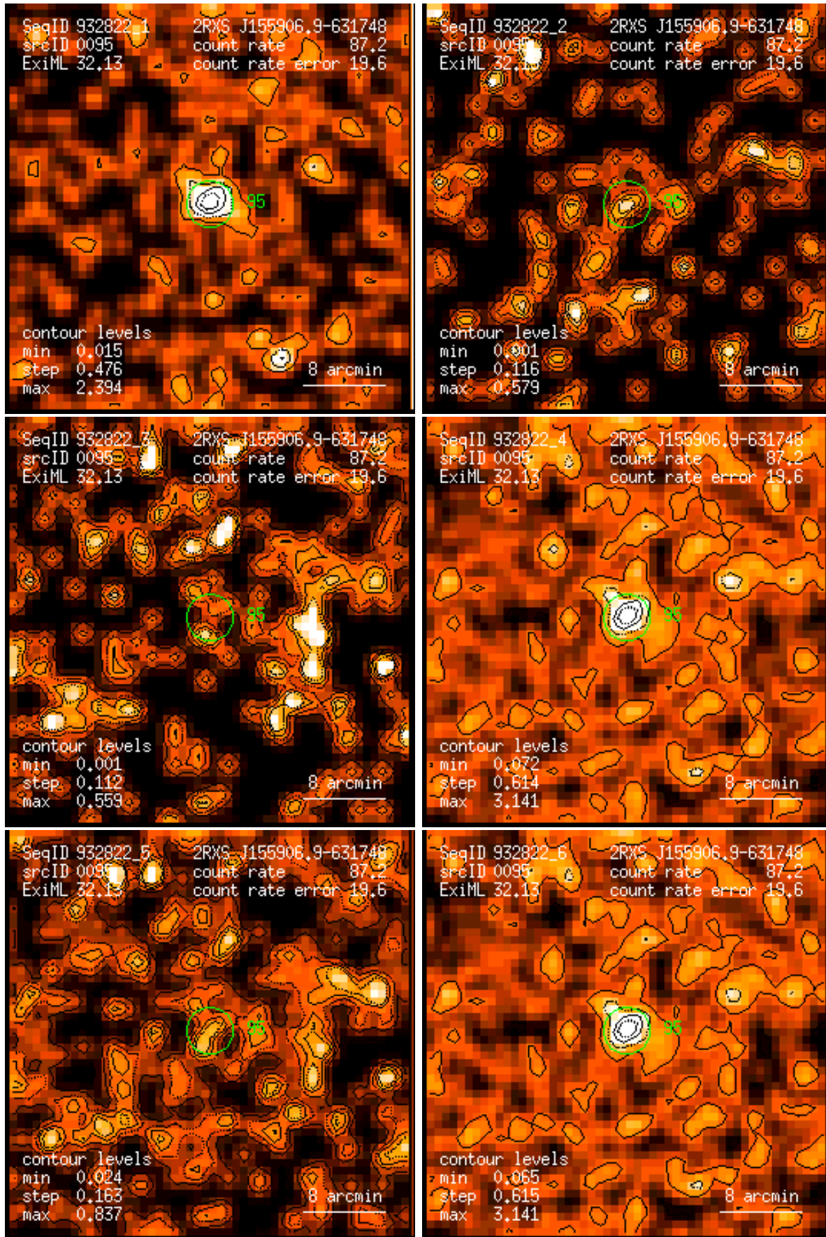
Figure 95: RASS 932822: detection 0095: band rate images, Gaussian filter: (1) PSPC channels 11 – 41, (2) 52 – 90, (3) 91 – 201, (4) 11 – 235, (5) 52 – 201, (6) 11 – 201. Broad band rates in counts/ks. Band rate contour levels in counts/ks/arcmin 2 .
