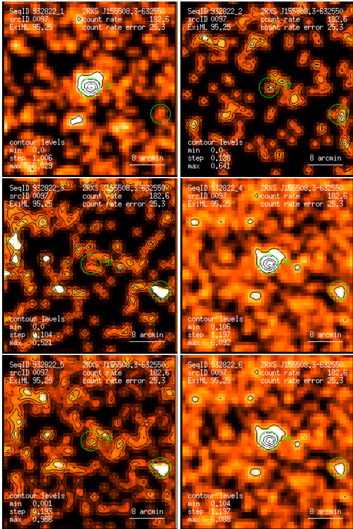
Figure 97: RASS 932822: detection 0097: band rate images, Gaussian filter: (1) PSPC channels 11 – 41, (2) 52 – 90, (3) 91 – 201, (4) 11 – 235, (5) 52 – 201, (6) 11 – 201. Broad band rates in counts/ks. Band rate contour levels in counts/ks/arcmin 2 .
