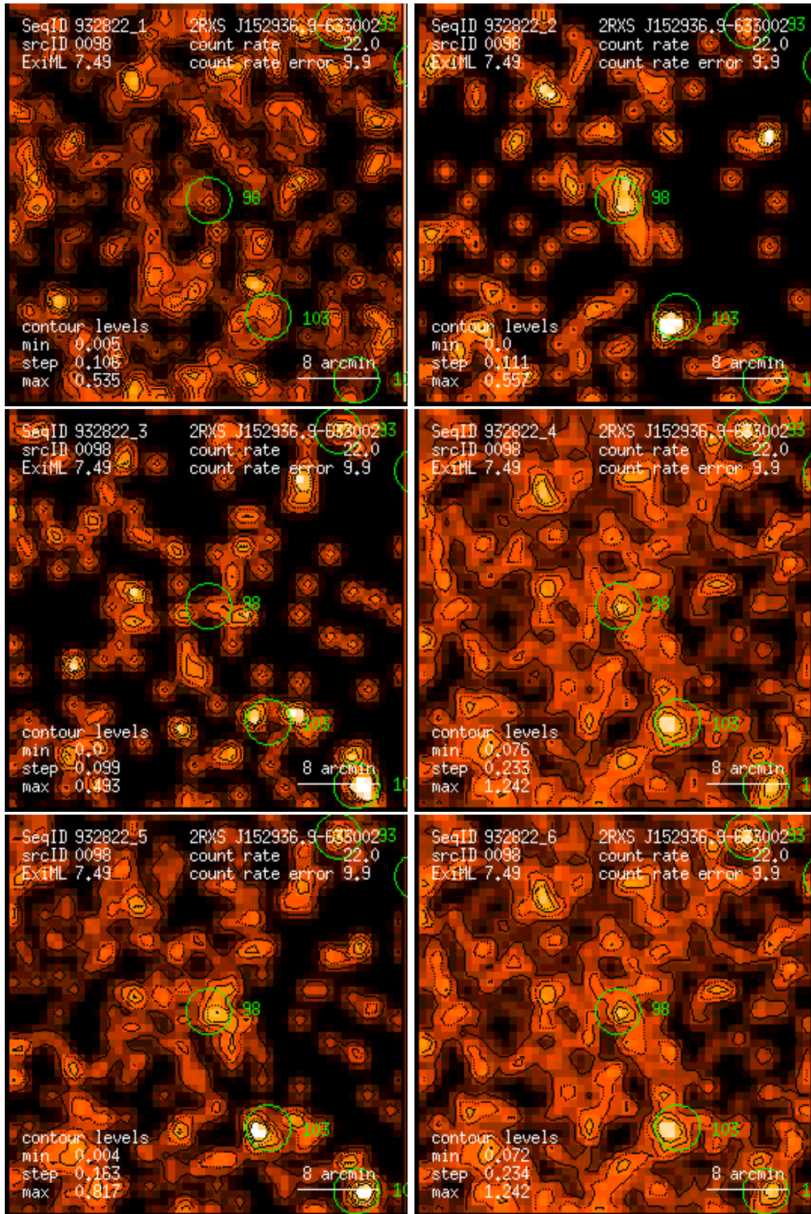
Figure 98: RASS 932822: detection 0098: band rate images, Gaussian filter: (1) PSPC channels 11 – 41, (2) 52 – 90, (3) 91 – 201, (4) 11 – 235, (5) 52 – 201, (6) 11 – 201. Broad band rates in counts/ks. Band rate contour levels in counts/ks/arcmin 2 .
