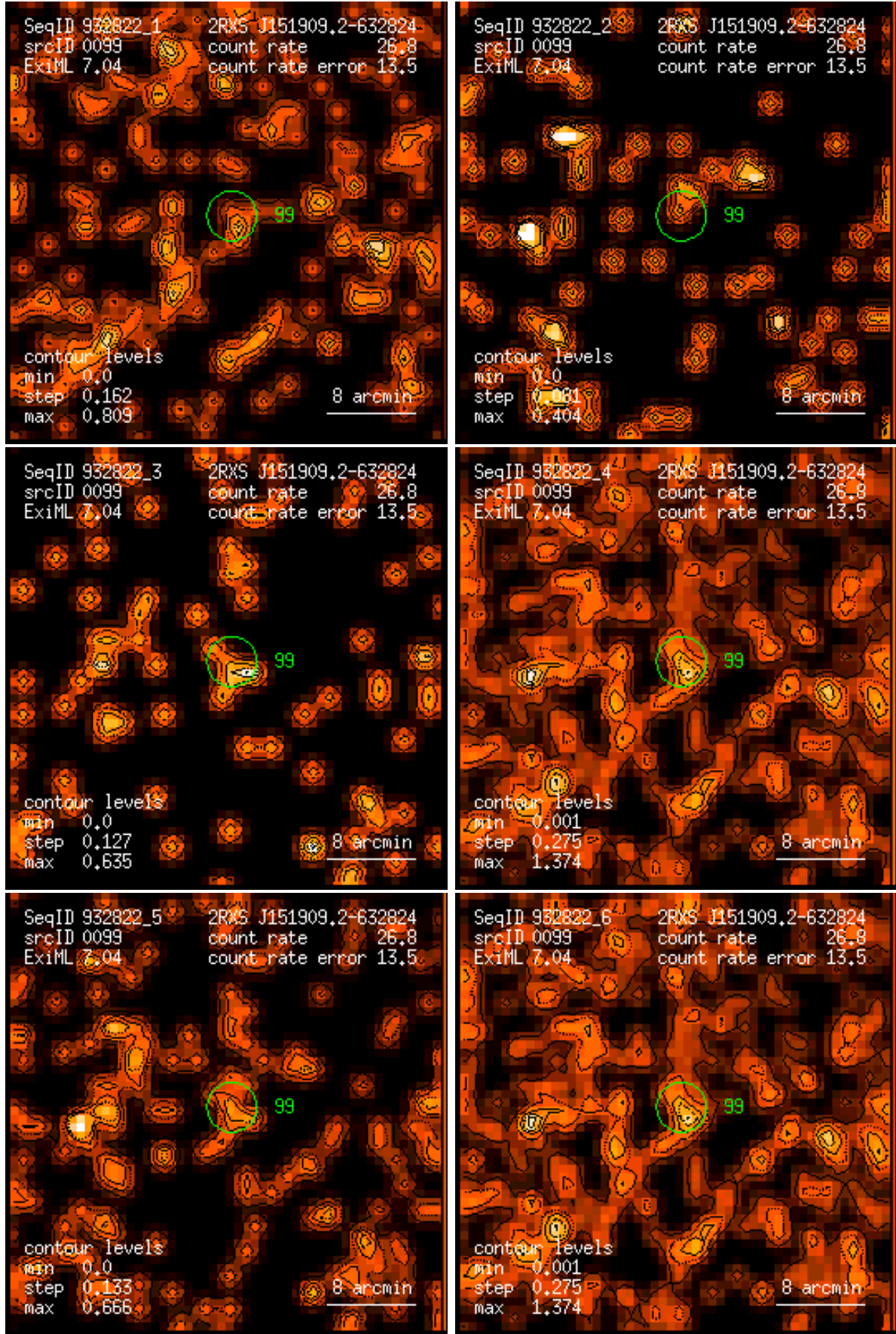
Figure 99: RASS 932822: detection 0099: band rate images, Gaussian filter: (1) PSPC channels 11 – 41, (2) 52 – 90, (3) 91 – 201, (4) 11 – 235, (5) 52 – 201, (6) 11 – 201. Broad band rates in counts/ks. Band rate contour levels in counts/ks/arcmin 2 .
