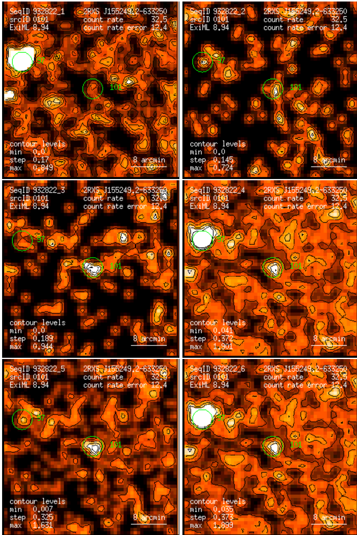
Figure 101: RASS 932822: detection 0101: band rate images, Gaussian filter: (1) PSPC channels 11 – 41, (2) 52 – 90, (3) 91 – 201, (4) 11 – 235, (5) 52 – 201, (6) 11 – 201. Broad band rates in counts/ks. Band rate contour levels in counts/ks/arcmin 2 .
