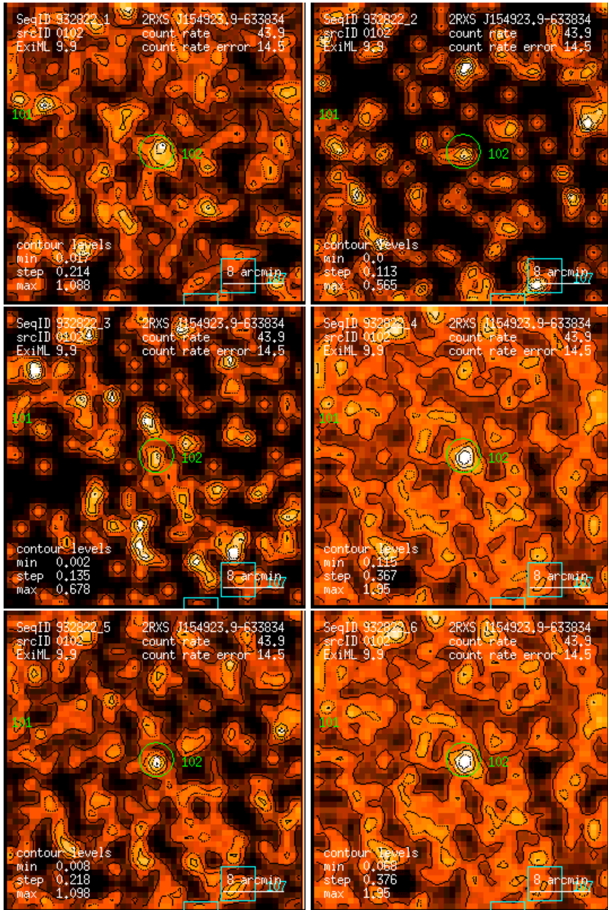
Figure 102: RASS 932822: detection 0102: band rate images, Gaussian filter: (1) PSPC channels 11 – 41, (2) 52 – 90, (3) 91 – 201, (4) 11 – 235, (5) 52 – 201, (6) 11 – 201. Broad band rates in counts/ks. Band rate contour levels in counts/ks/arcmin 2 .
