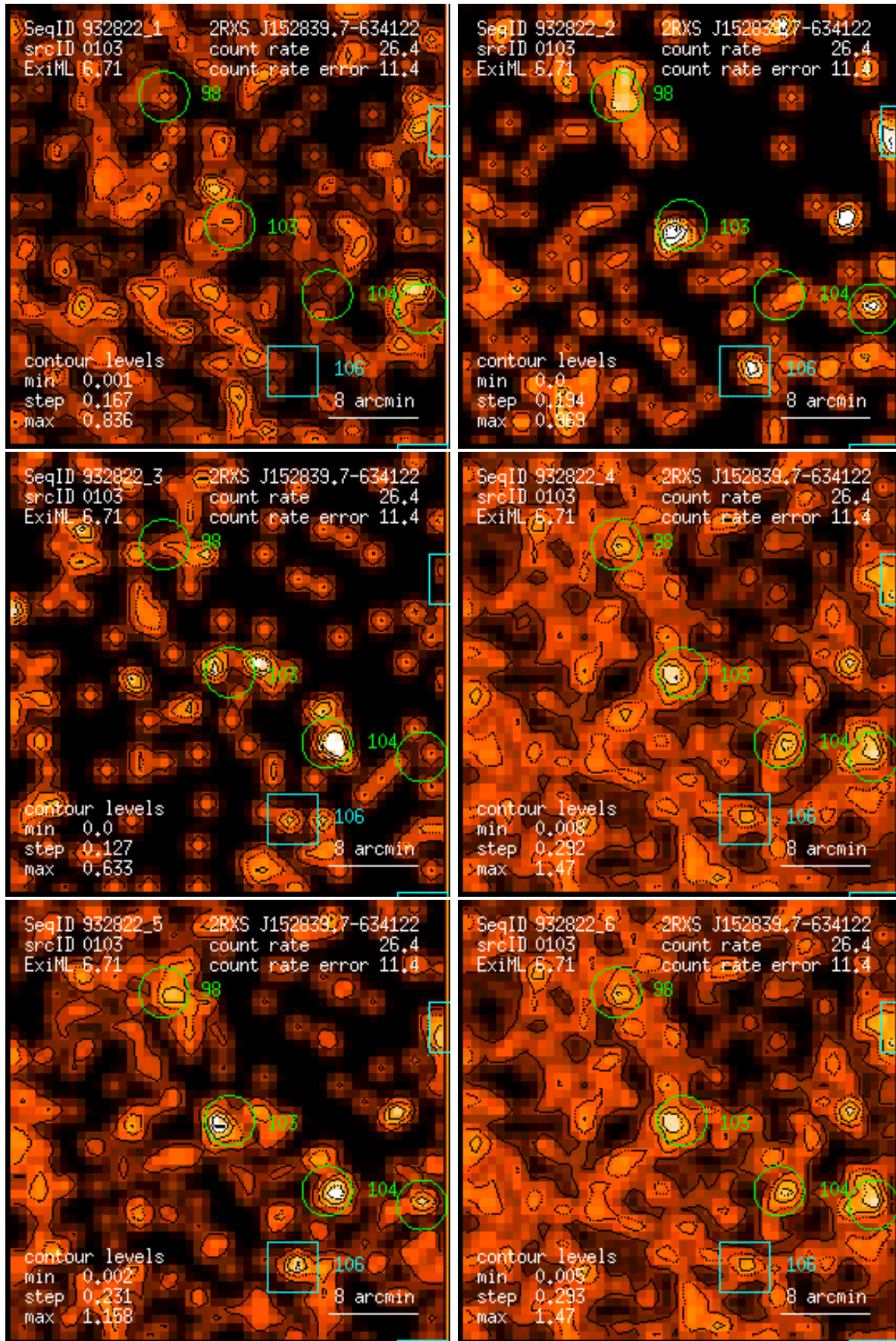
Figure 103: RASS 932822: detection 0103: band rate images, Gaussian filter: (1) PSPC channels 11 – 41, (2) 52 – 90, (3) 91 – 201, (4) 11 – 235, (5) 52 – 201, (6) 11 – 201. Broad band rates in counts/ks. Band rate contour levels in counts/ks/arcmin 2 .
