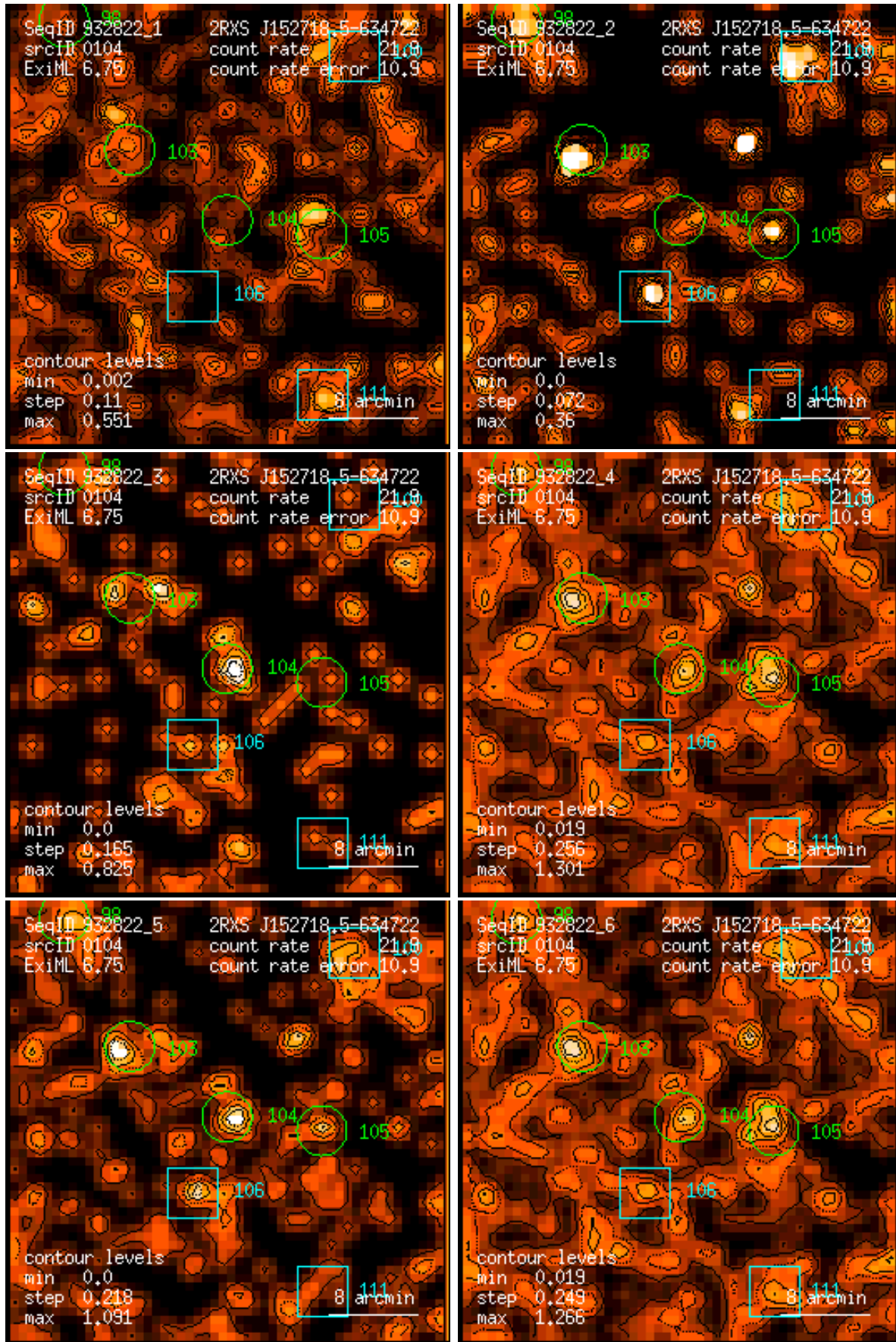
Figure 104: RASS 932822: detection 0104: band rate images, Gaussian filter: (1) PSPC channels 11 – 41, (2) 52 – 90, (3) 91 – 201, (4) 11 – 235, (5) 52 – 201, (6) 11 – 201. Broad band rates in counts/ks. Band rate contour levels in counts/ks/arcmin 2 .
