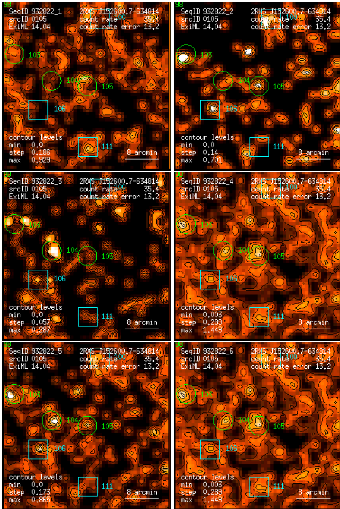
Figure 105: RASS 932822: detection 0105: band rate images, Gaussian filter: (1) PSPC channels 11 – 41, (2) 52 – 90, (3) 91 – 201, (4) 11 – 235, (5) 52 – 201, (6) 11 – 201. Broad band rates in counts/ks. Band rate contour levels in counts/ks/arcmin 2 .
