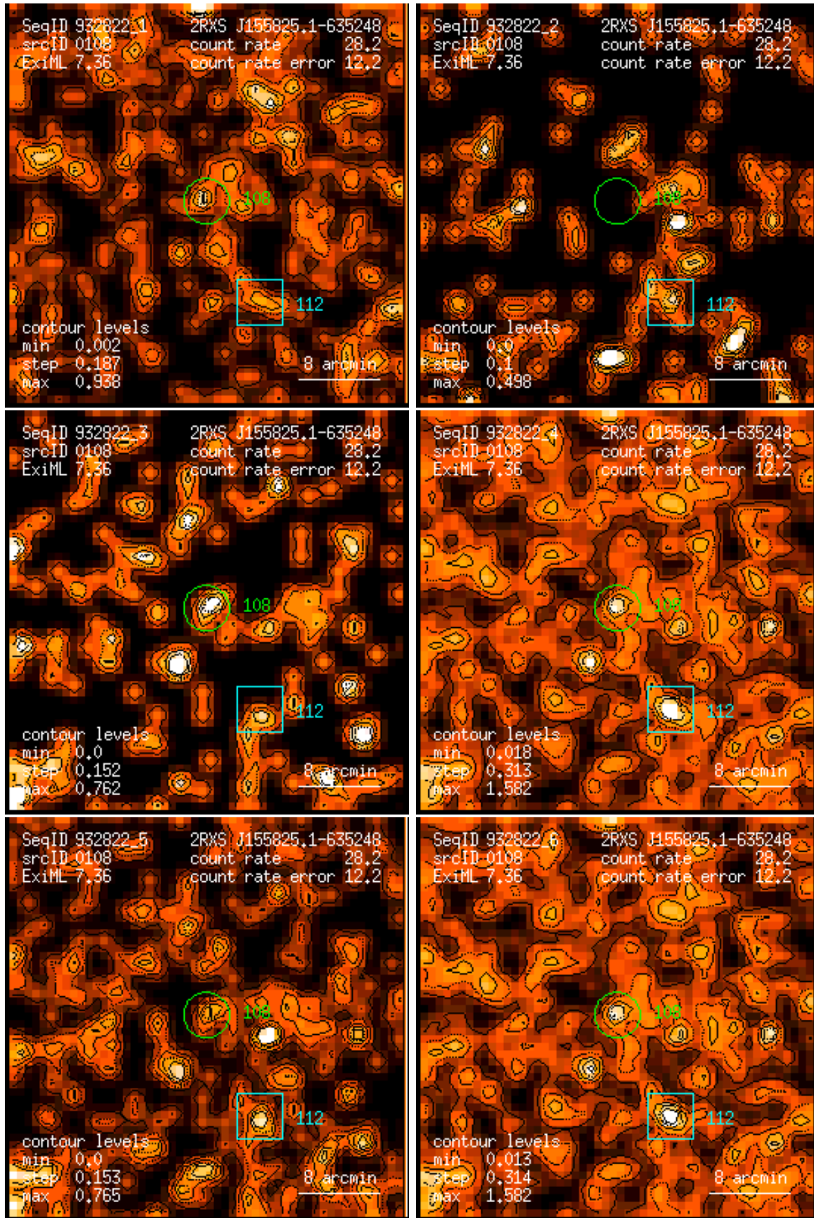
Figure 108: RASS 932822: detection 0108: band rate images, Gaussian filter: (1) PSPC channels 11 – 41, (2) 52 – 90, (3) 91 – 201, (4) 11 – 235, (5) 52 – 201, (6) 11 – 201. Broad band rates in counts/ks. Band rate contour levels in counts/ks/arcmin 2 .
