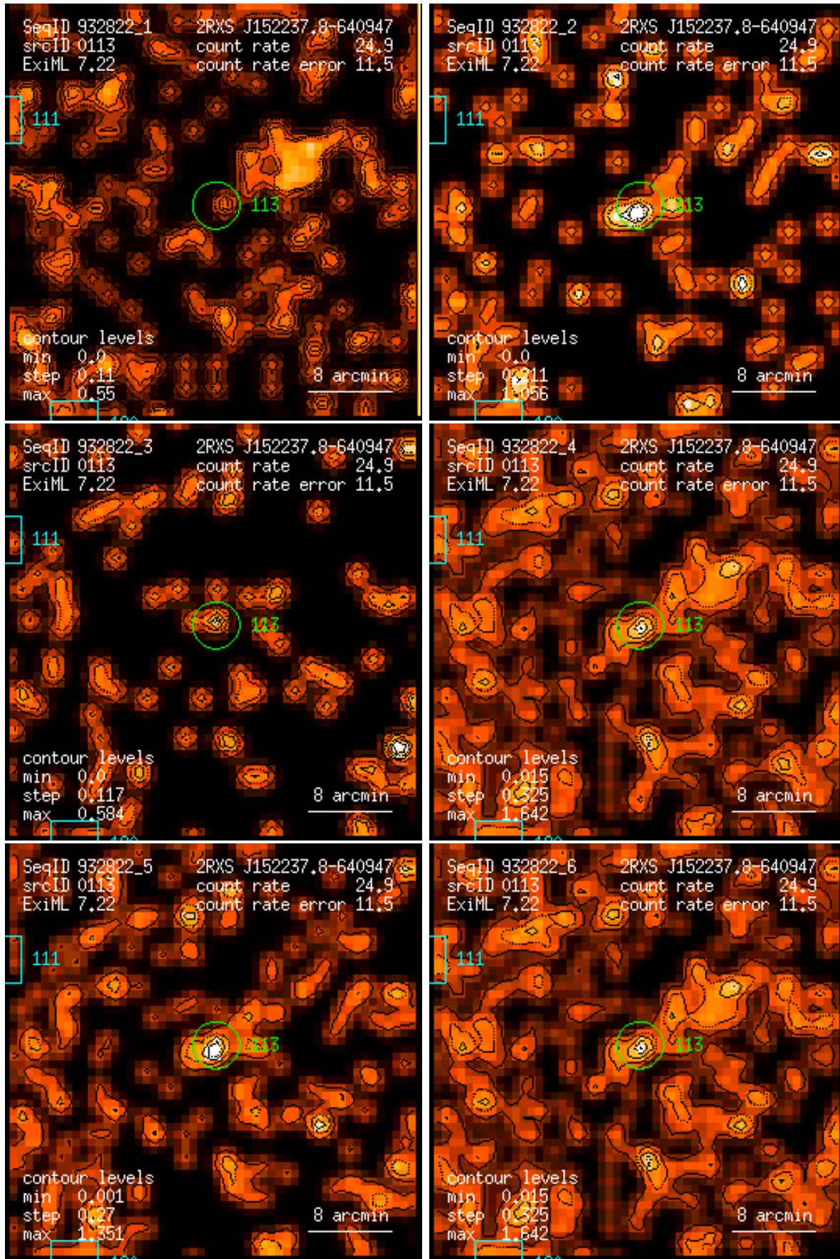
Figure 113: RASS 932822: detection 0113: band rate images, Gaussian filter: (1) PSPC channels 11 – 41, (2) 52 – 90, (3) 91 – 201, (4) 11 – 235, (5) 52 – 201, (6) 11 – 201. Broad band rates in counts/ks. Band rate contour levels in counts/ks/arcmin 2 .
