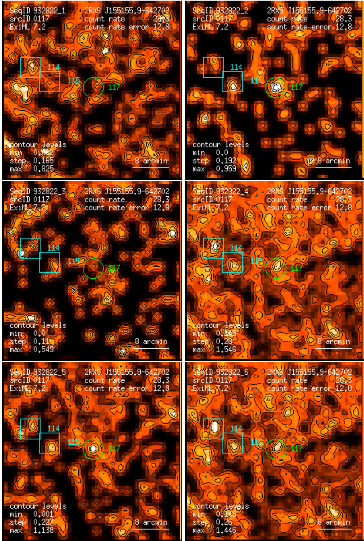
Figure 117: RASS 932822: detection 0117: band rate images, Gaussian filter: (1) PSPC channels 11 – 41, (2) 52 – 90, (3) 91 – 201, (4) 11 – 235, (5) 52 – 201, (6) 11 – 201. Broad band rates in counts/ks. Band rate contour levels in counts/ks/arcmin 2 .
