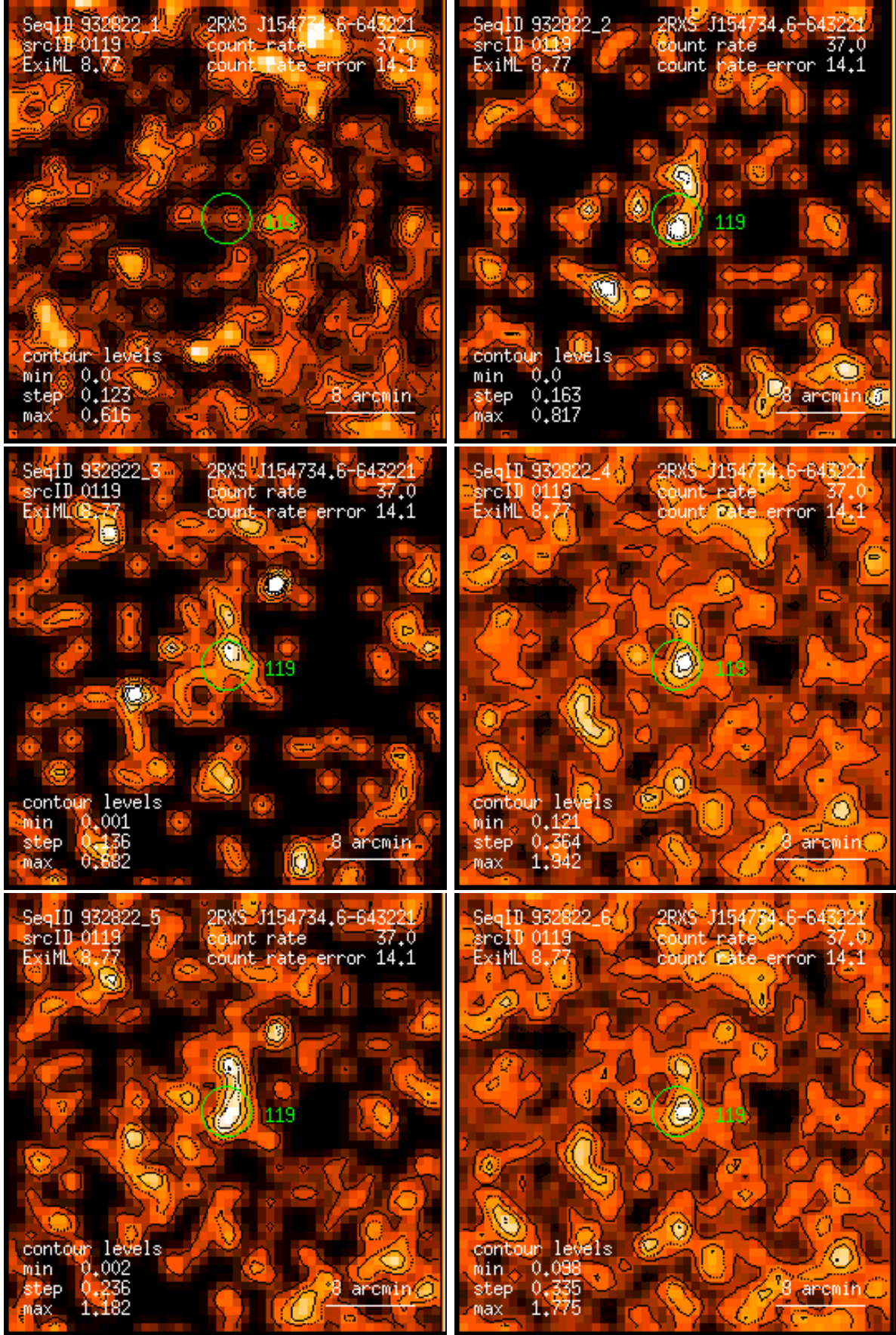
Figure 119: RASS 932822: detection 0119: band rate images, Gaussian filter: (1) PSPC channels 11 – 41, (2) 52 – 90, (3) 91 – 201, (4) 11 – 235, (5) 52 – 201, (6) 11 – 201. Broad band rates in counts/ks. Band rate contour levels in counts/ks/arcmin 2 .
