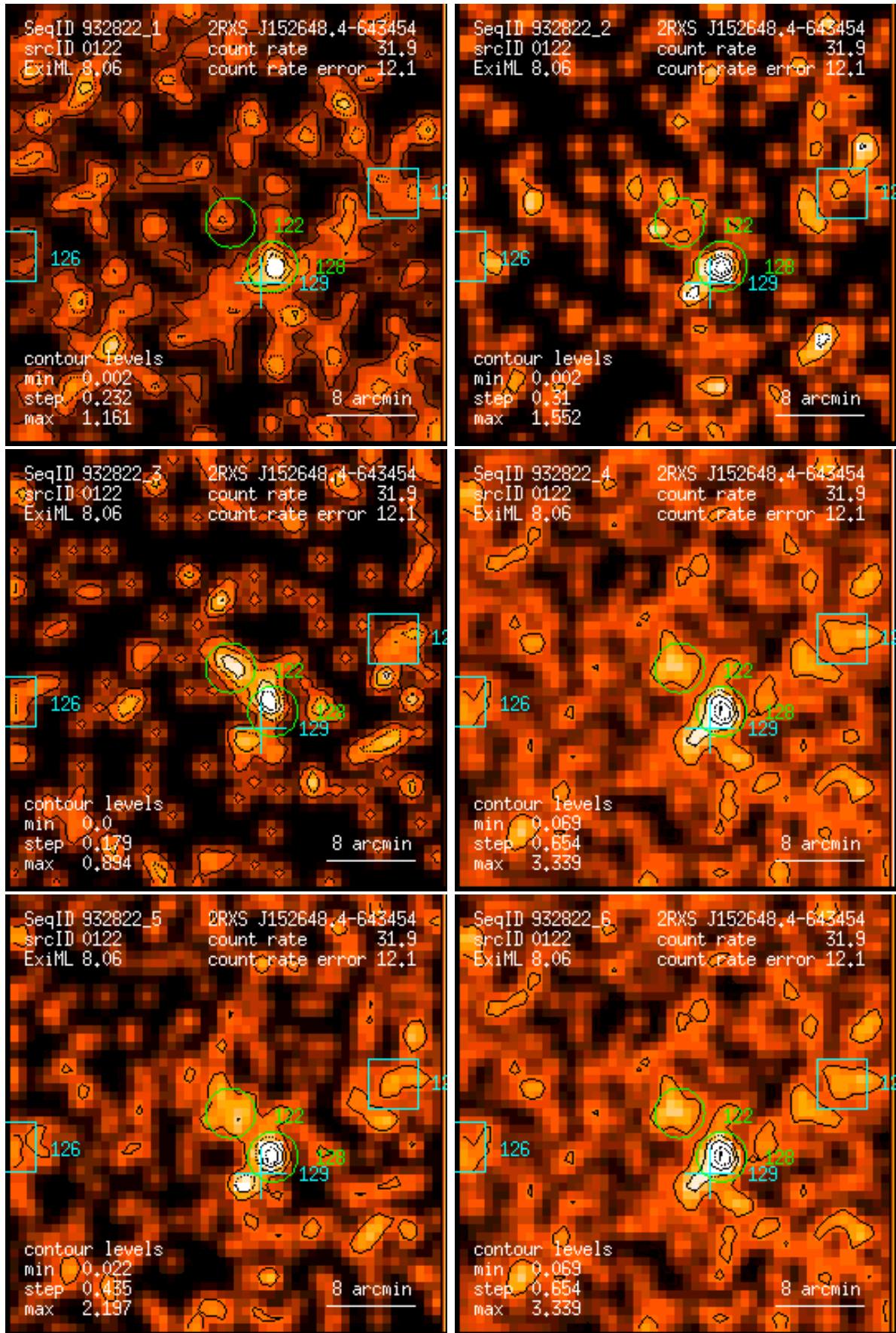
Figure 122: RASS 932822: detection 0122: band rate images, Gaussian filter: (1) PSPC channels 11 – 41, (2) 52 – 90, (3) 91 – 201, (4) 11 – 235, (5) 52 – 201, (6) 11 – 201. Broad band rates in counts/ks. Band rate contour levels in counts/ks/arcmin 2 .
