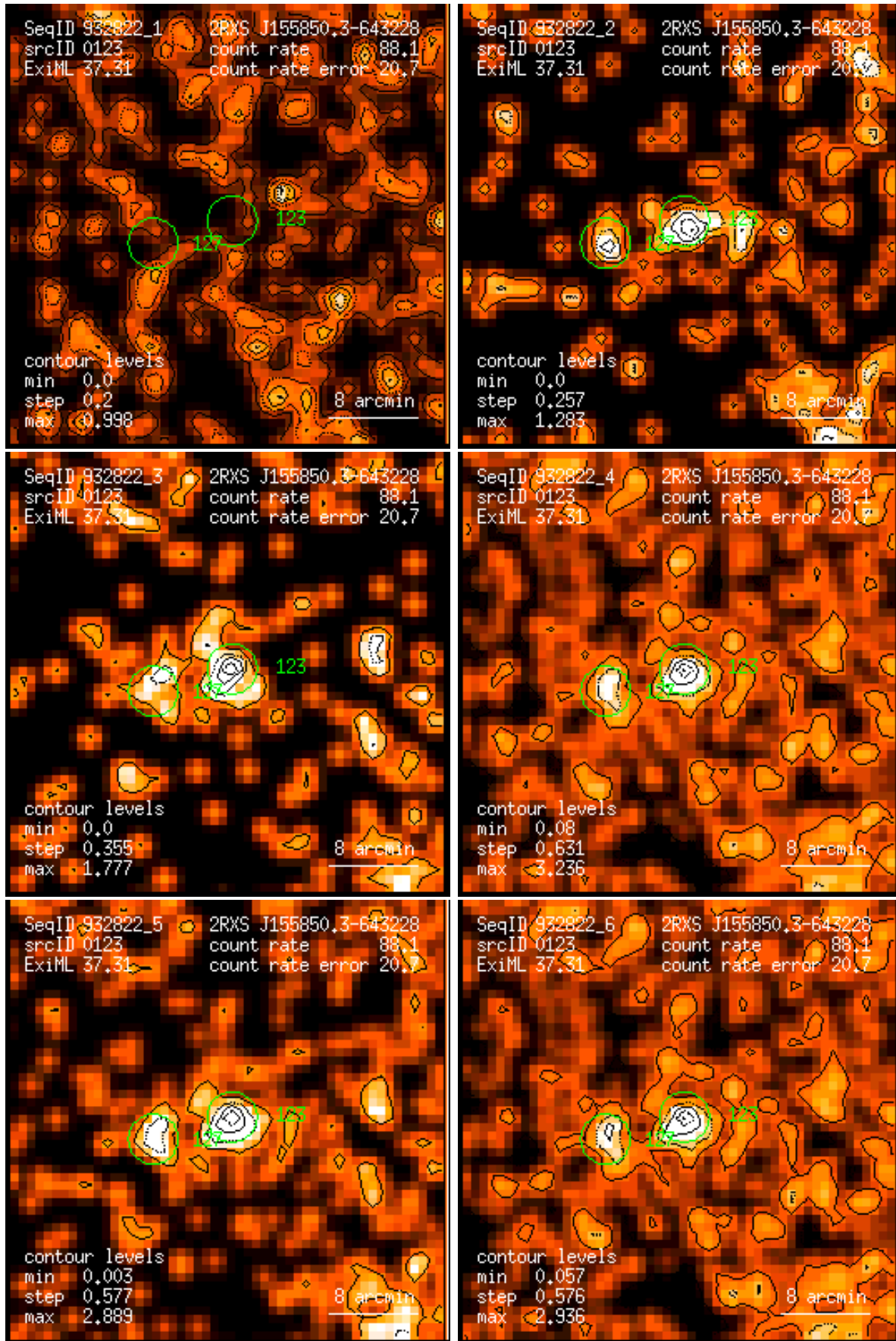
Figure 123: RASS 932822: detection 0123: band rate images, Gaussian filter: (1) PSPC channels 11 – 41, (2) 52 – 90, (3) 91 – 201, (4) 11 – 235, (5) 52 – 201, (6) 11 – 201. Broad band rates in counts/ks. Band rate contour levels in counts/ks/arcmin 2 .
