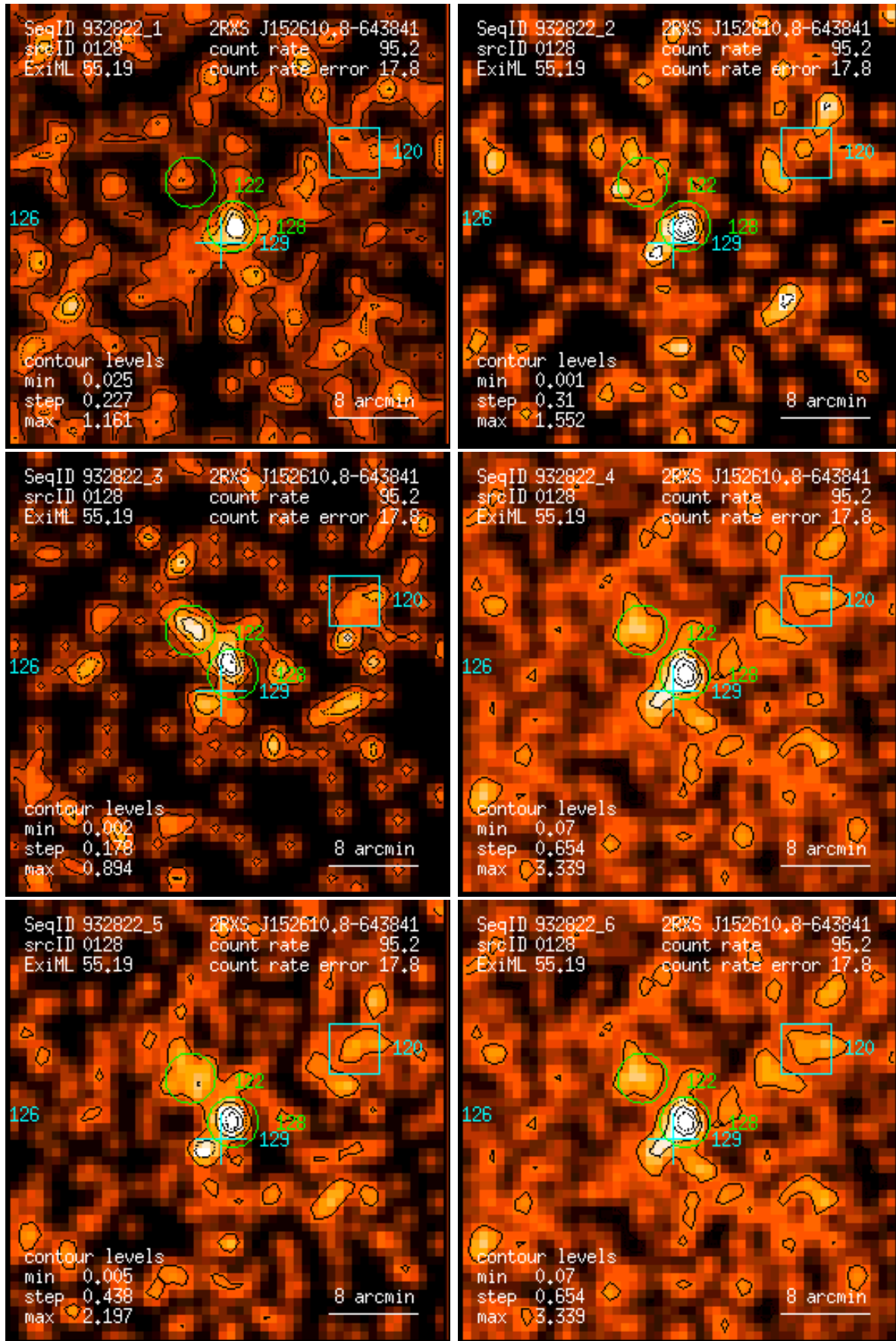
Figure 128: RASS 932822: detection 0128: band rate images, Gaussian filter: (1) PSPC channels 11 – 41, (2) 52 – 90, (3) 91 – 201, (4) 11 – 235, (5) 52 – 201, (6) 11 – 201. Broad band rates in counts/ks. Band rate contour levels in counts/ks/arcmin 2 .
