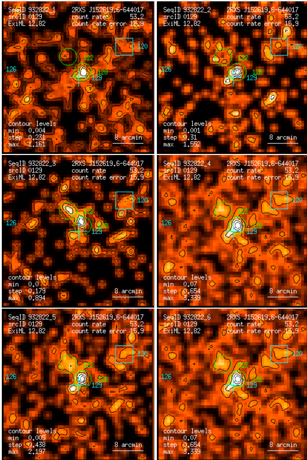
Figure 129: RASS 932822: detection 0129: band rate images, Gaussian filter: (1) PSPC channels 11 – 41, (2) 52 – 90, (3) 91 – 201, (4) 11 – 235, (5) 52 – 201, (6) 11 – 201. Broad band rates in counts/ks. Band rate contour levels in counts/ks/arcmin 2 .
