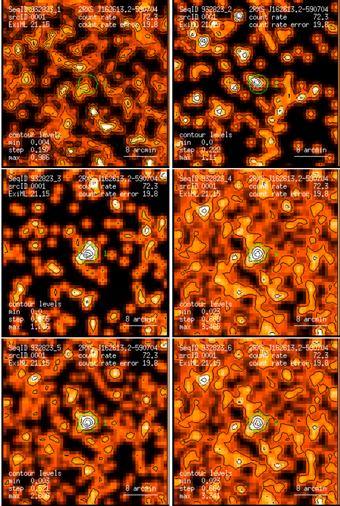
Figure 1: RASS 932823: detection 0001: band rate images, Gaussian filter: (1) PSPC channels 11 – 41, (2) 52 – 90, (3) 91 – 201, (4) 11 – 235, (5) 52 – 201, (6) 11 – 201. Broad band rates in counts/ks. Band rate contour levels in counts/ks/arcmin 2 .
