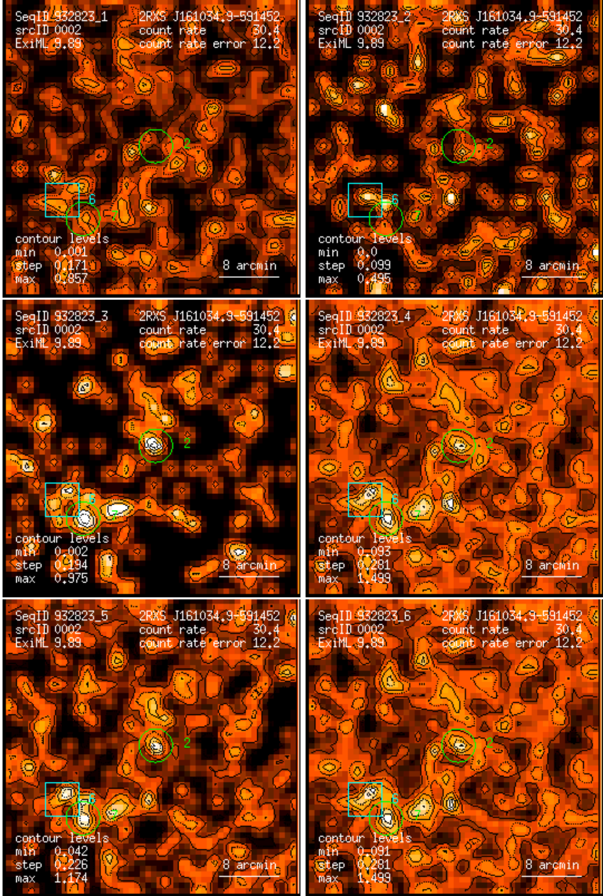
Figure 2: RASS 932823: detection 0002: band rate images, Gaussian filter: (1) PSPC channels 11 – 41, (2) 52 – 90, (3) 91 – 201, (4) 11 – 235, (5) 52 – 201, (6) 11 – 201. Broad band rates in counts/ks. Band rate contour levels in counts/ks/arcmin 2 .
