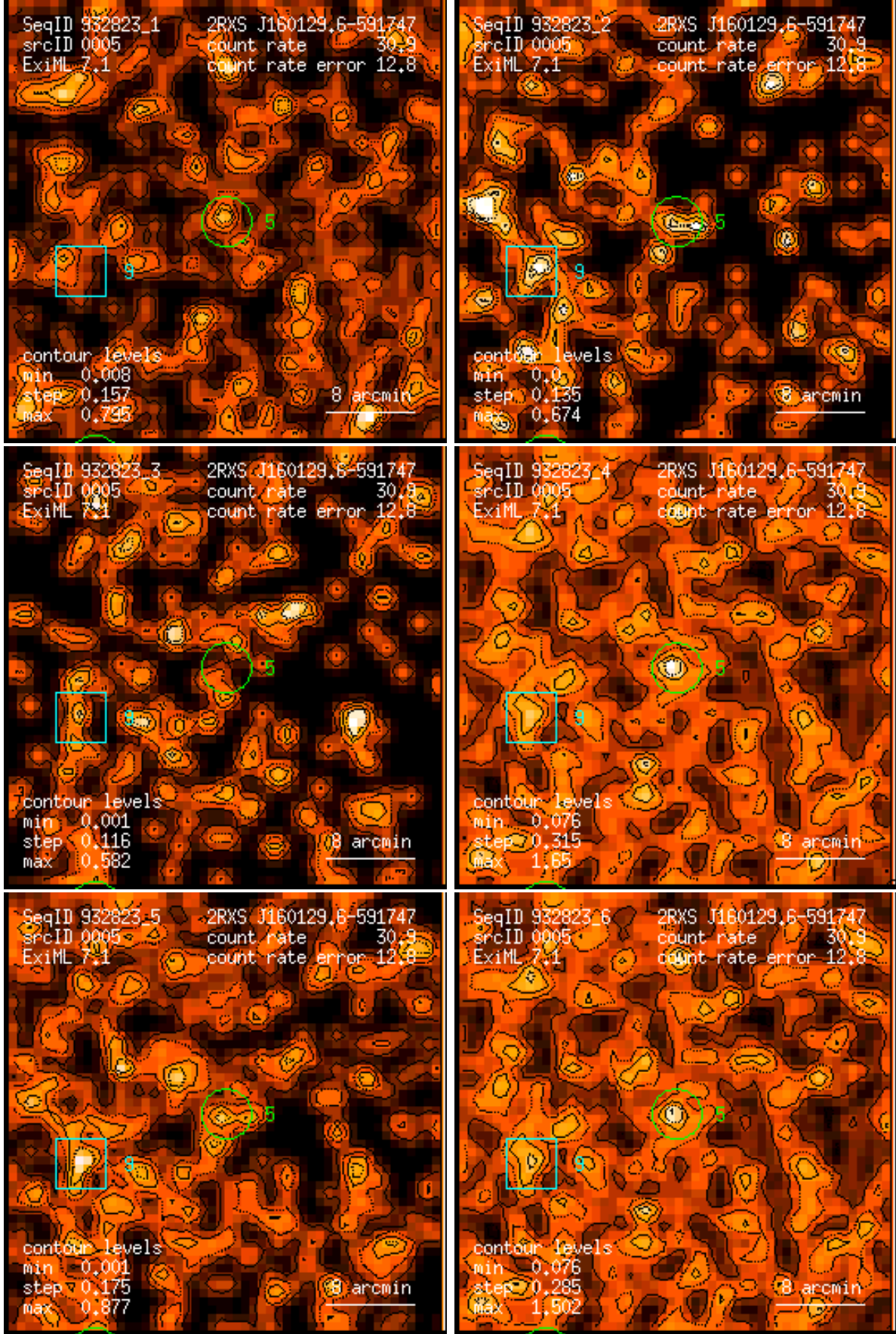
Figure 5: RASS 932823: detection 0005: band rate images, Gaussian filter: (1) PSPC channels 11 – 41, (2) 52 – 90, (3) 91 – 201, (4) 11 – 235, (5) 52 – 201, (6) 11 – 201. Broad band rates in counts/ks. Band rate contour levels in counts/ks/arcmin 2 .
