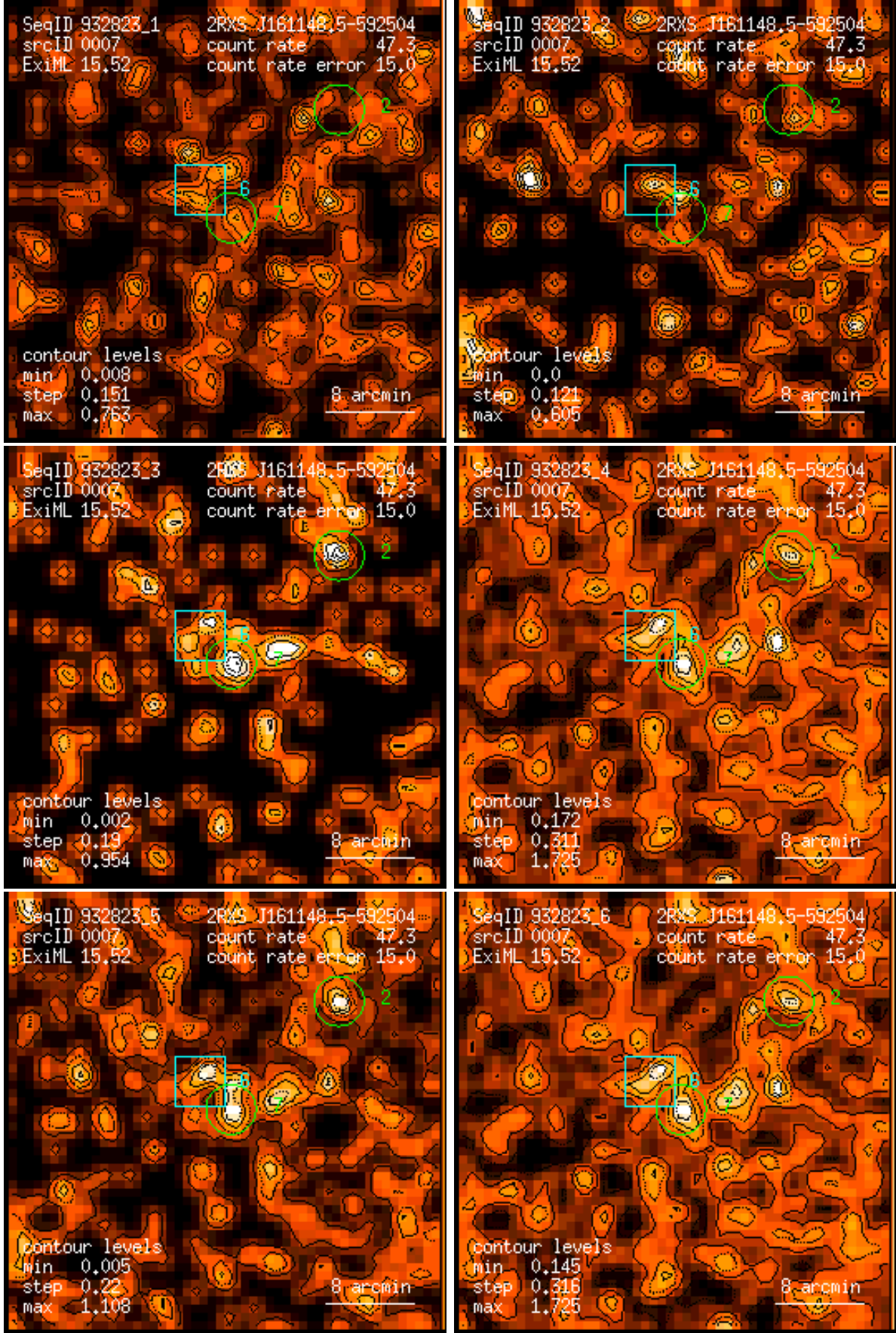
Figure 7: RASS 932823: detection 0007: band rate images, Gaussian filter: (1) PSPC channels 11 – 41, (2) 52 – 90, (3) 91 – 201, (4) 11 – 235, (5) 52 – 201, (6) 11 – 201. Broad band rates in counts/ks. Band rate contour levels in counts/ks/arcmin 2 .
