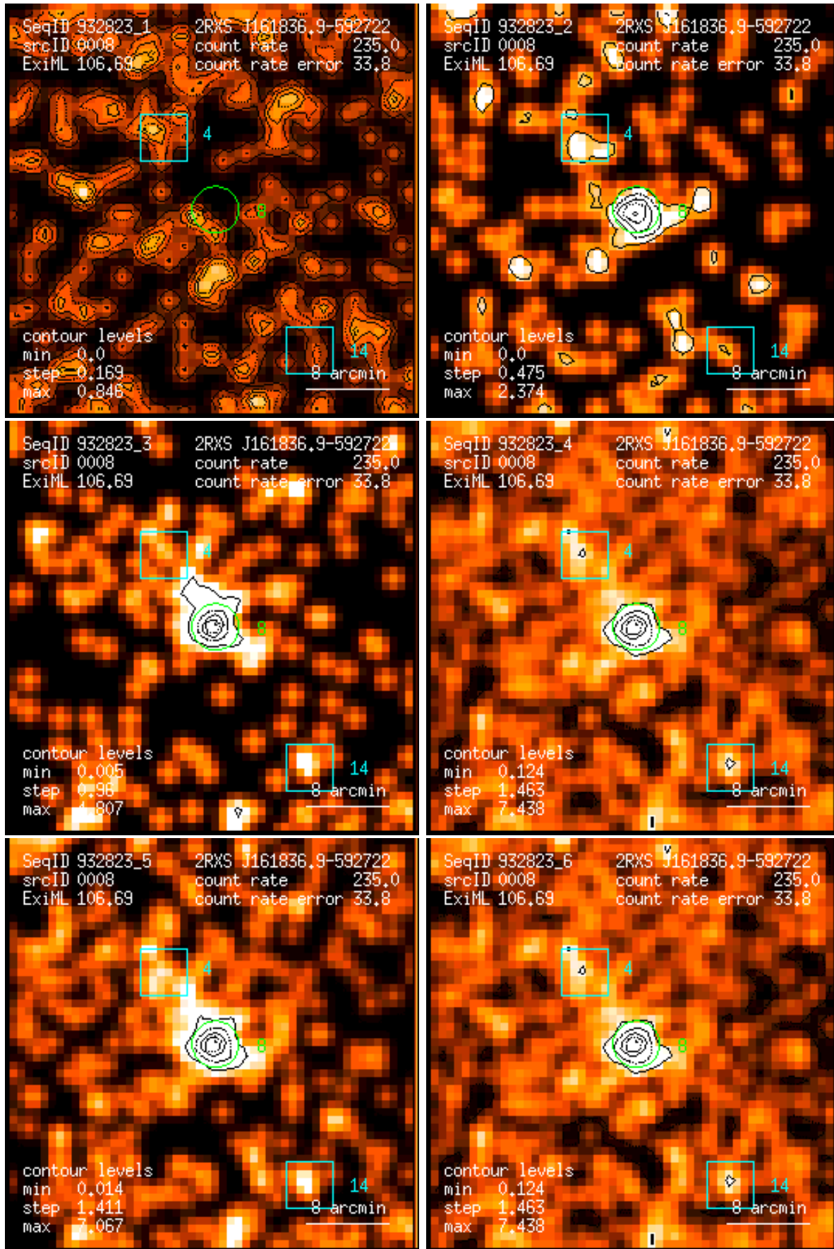
Figure 8: RASS 932823: detection 0008: band rate images, Gaussian filter: (1) PSPC channels 11 – 41, (2) 52 – 90, (3) 91 – 201, (4) 11 – 235, (5) 52 – 201, (6) 11 – 201. Broad band rates in counts/ks. Band rate contour levels in counts/ks/arcmin 2 .
