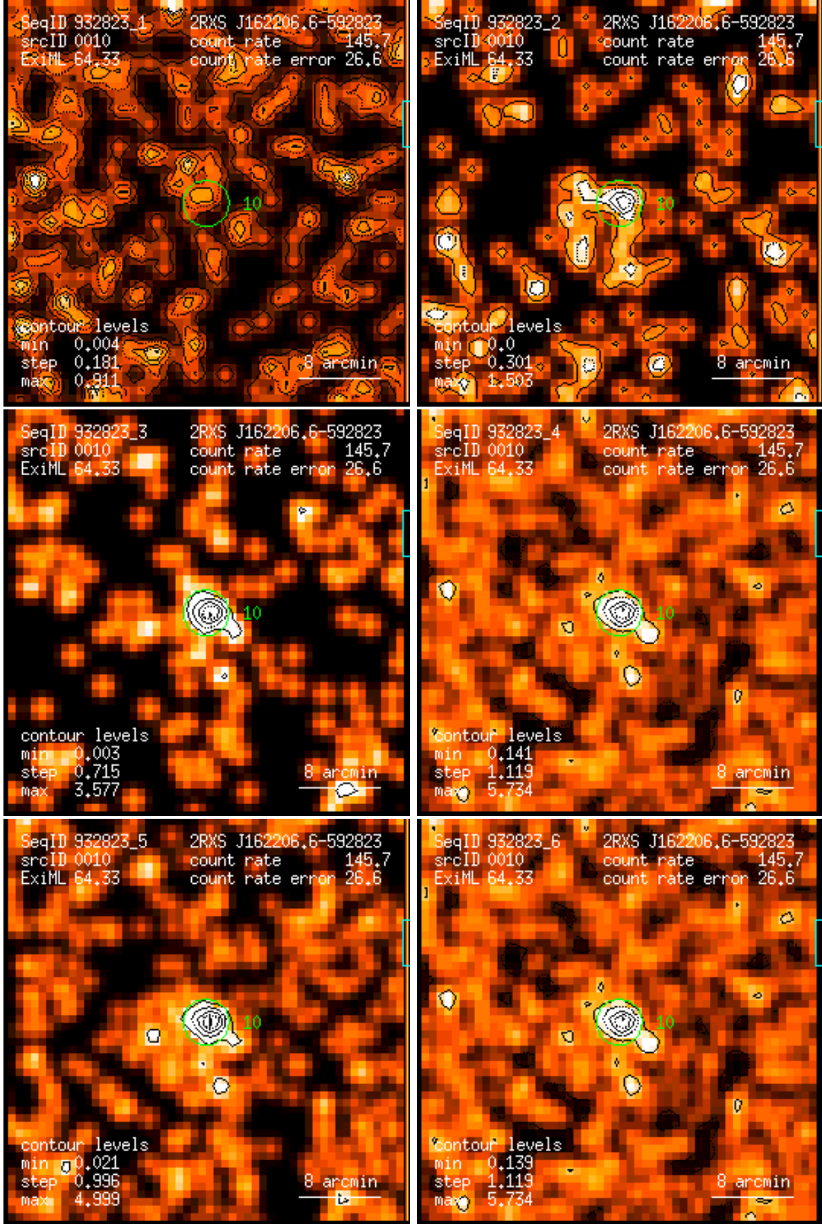
Figure 10: RASS 932823: detection 0010: band rate images, Gaussian filter: (1) PSPC channels 11 – 41, (2) 52 – 90, (3) 91 – 201, (4) 11 – 235, (5) 52 – 201, (6) 11 – 201. Broad band rates in counts/ks. Band rate contour levels in counts/ks/arcmin 2 .
