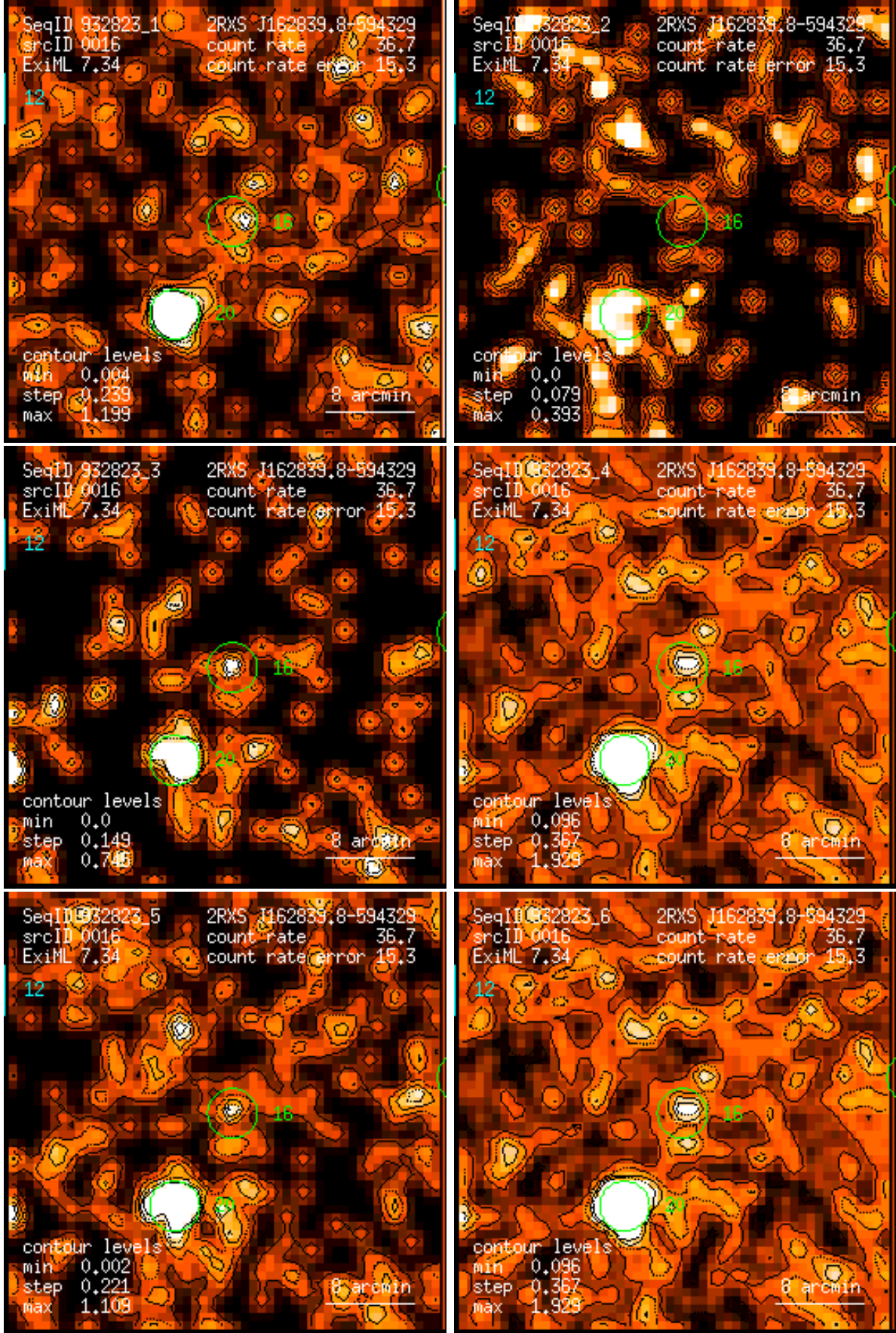
Figure 16: RASS 932823: detection 0016: band rate images, Gaussian filter: (1) PSPC channels 11 – 41, (2) 52 – 90, (3) 91 – 201, (4) 11 – 235, (5) 52 – 201, (6) 11 – 201. Broad band rates in counts/ks. Band rate contour levels in counts/ks/arcmin 2 .
