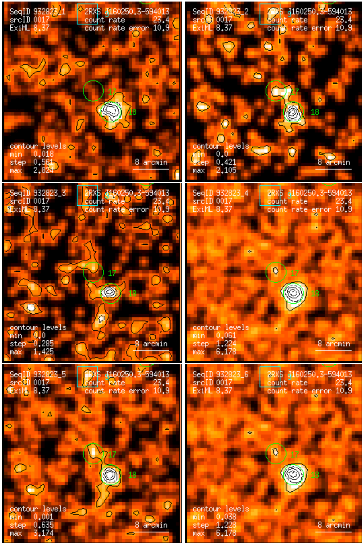
Figure 17: RASS 932823: detection 0017: band rate images, Gaussian filter: (1) PSPC channels 11 – 41, (2) 52 – 90, (3) 91 – 201, (4) 11 – 235, (5) 52 – 201, (6) 11 – 201. Broad band rates in counts/ks. Band rate contour levels in counts/ks/arcmin 2 .
