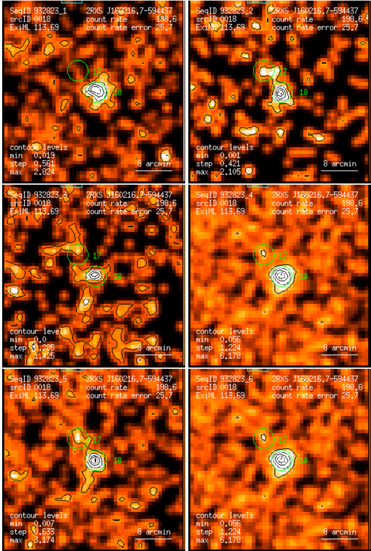
Figure 18: RASS 932823: detection 0018: band rate images, Gaussian filter: (1) PSPC channels 11 – 41, (2) 52 – 90, (3) 91 – 201, (4) 11 – 235, (5) 52 – 201, (6) 11 – 201. Broad band rates in counts/ks. Band rate contour levels in counts/ks/arcmin 2 .
