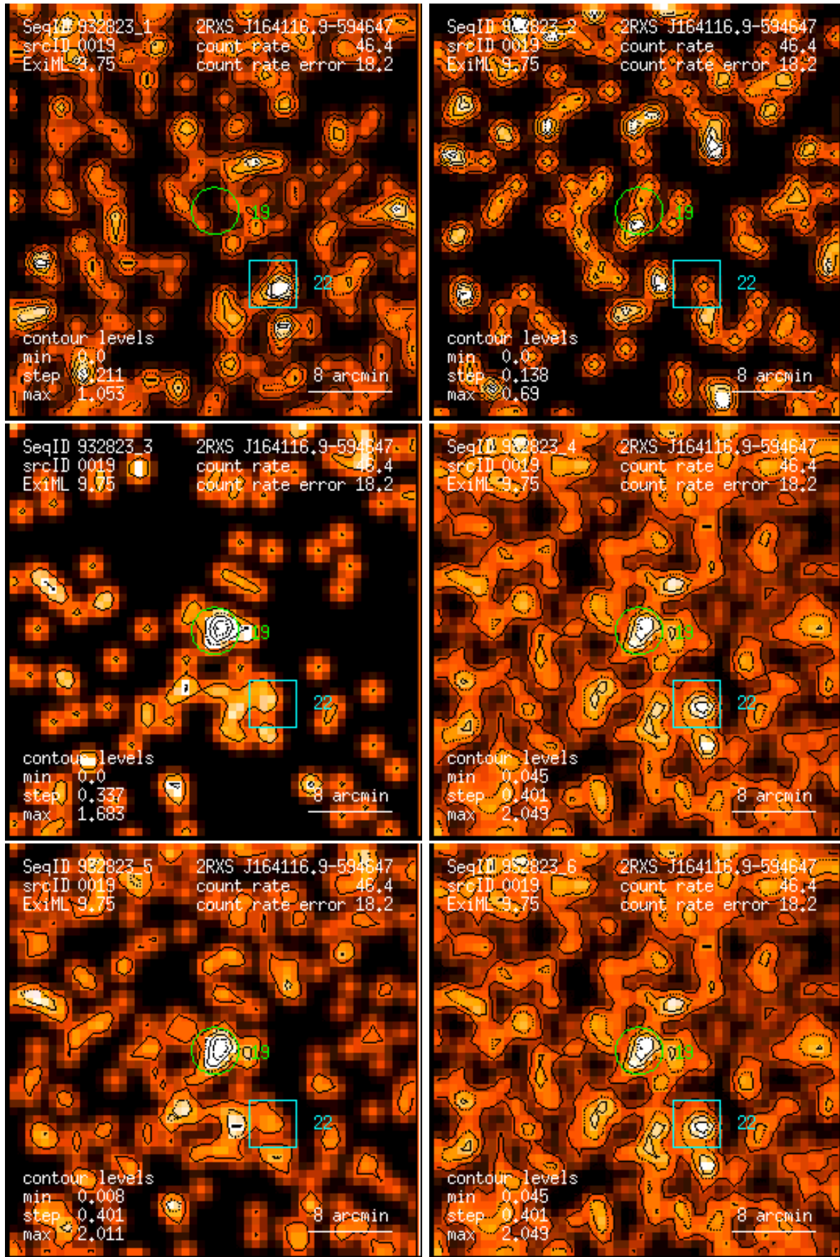
Figure 19: RASS 932823: detection 0019: band rate images, Gaussian filter: (1) PSPC channels 11 – 41, (2) 52 – 90, (3) 91 – 201, (4) 11 – 235, (5) 52 – 201, (6) 11 – 201. Broad band rates in counts/ks. Band rate contour levels in counts/ks/arcmin 2 .
