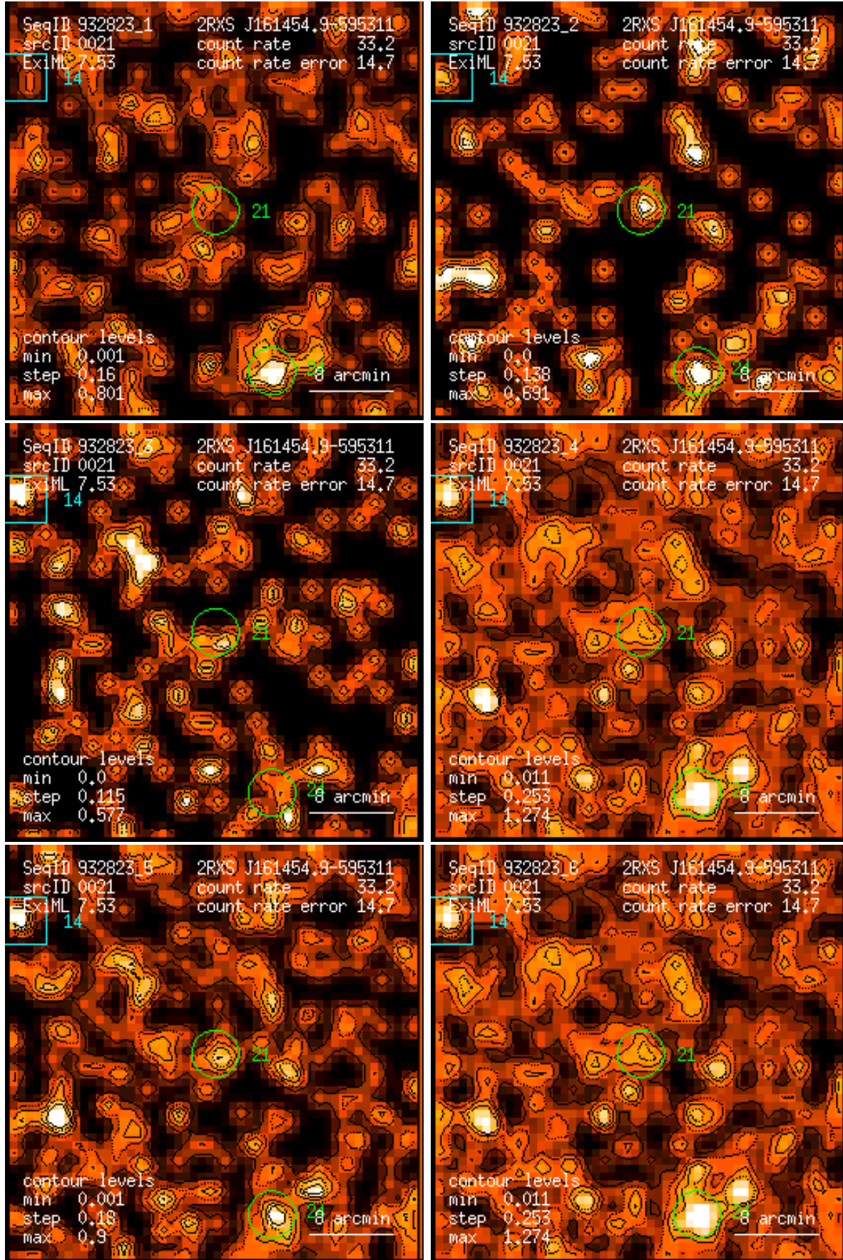
Figure 21: RASS 932823: detection 0021: band rate images, Gaussian filter: (1) PSPC channels 11 – 41, (2) 52 – 90, (3) 91 – 201, (4) 11 – 235, (5) 52 – 201, (6) 11 – 201. Broad band rates in counts/ks. Band rate contour levels in counts/ks/arcmin 2 .
