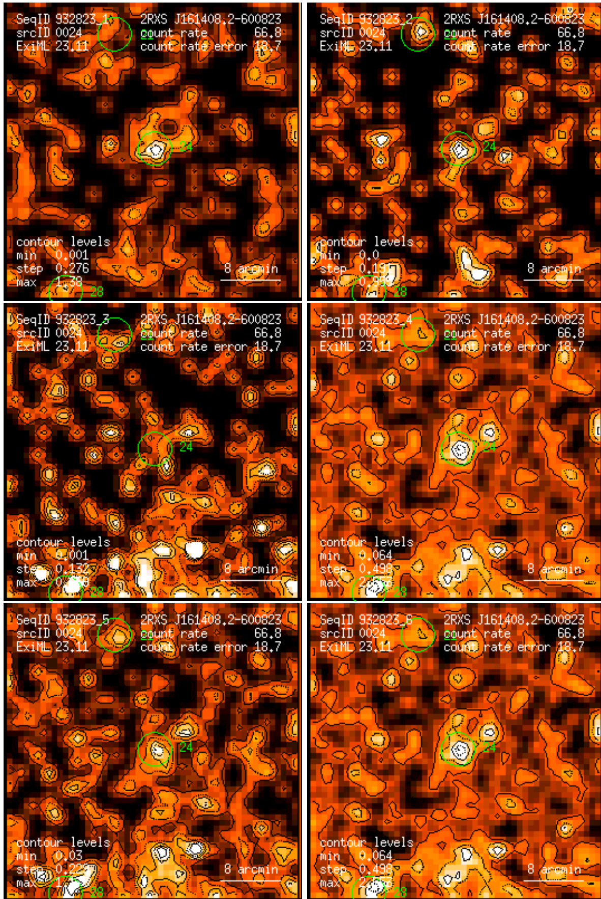
Figure 24: RASS 932823: detection 0024: band rate images, Gaussian filter: (1) PSPC channels 11 – 41, (2) 52 – 90, (3) 91 – 201, (4) 11 – 235, (5) 52 – 201, (6) 11 – 201. Broad band rates in counts/ks. Band rate contour levels in counts/ks/arcmin 2 .
