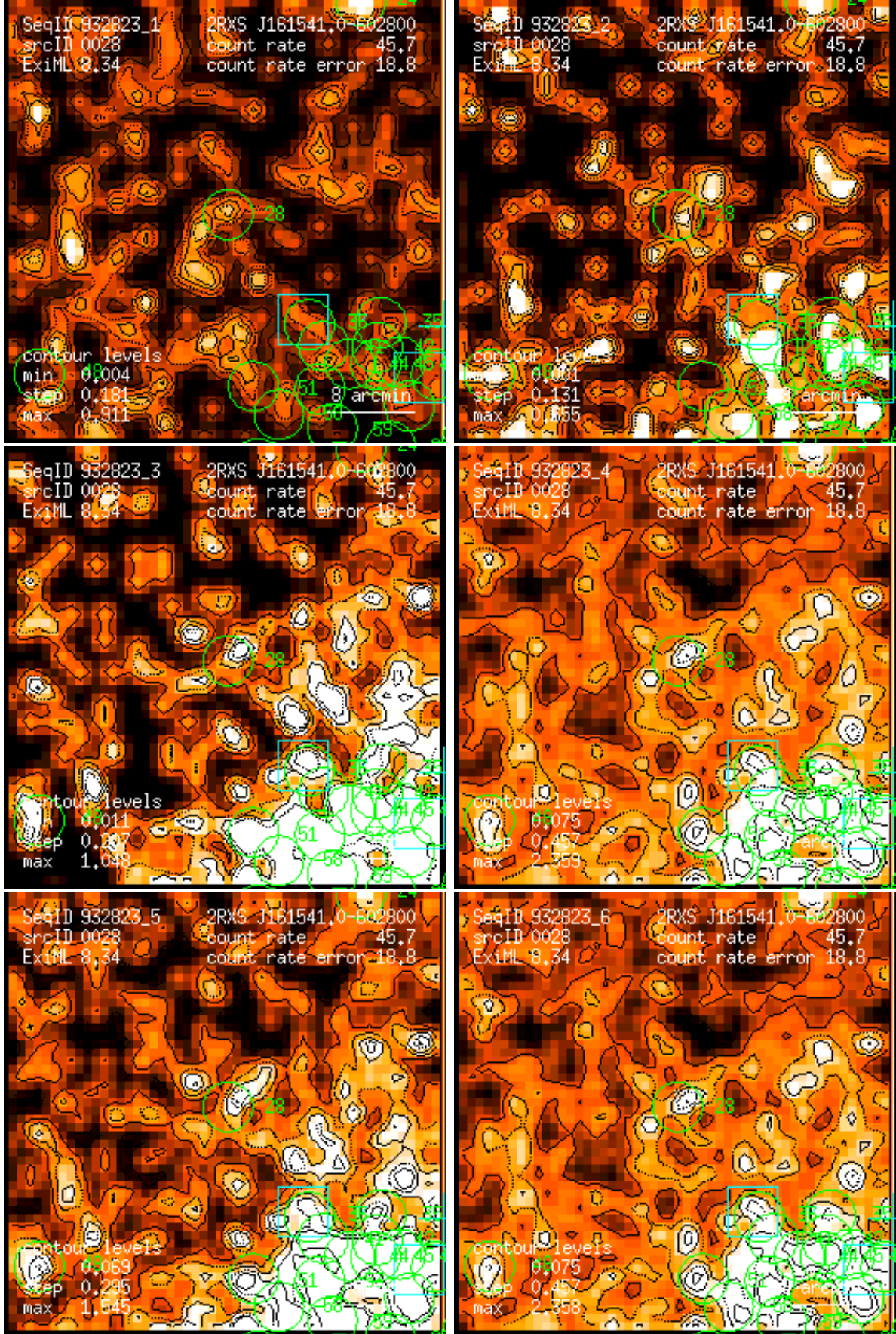
Figure 28: RASS 932823: detection 0028: band rate images, Gaussian filter: (1) PSPC channels 11 – 41, (2) 52 – 90, (3) 91 – 201, (4) 11 – 235, (5) 52 – 201, (6) 11 – 201. Broad band rates in counts/ks. Band rate contour levels in counts/ks/arcmin 2 .
