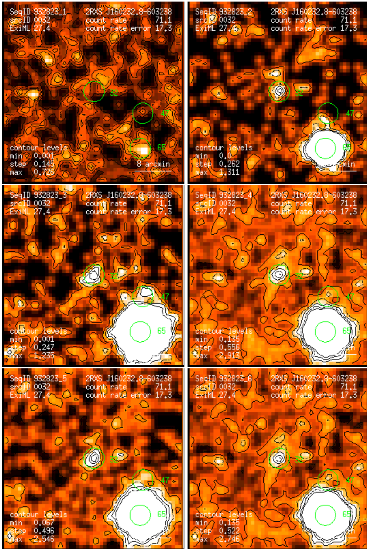
Figure 32: RASS 932823: detection 0032: band rate images, Gaussian filter: (1) PSPC channels 11 – 41, (2) 52 – 90, (3) 91 – 201, (4) 11 – 235, (5) 52 – 201, (6) 11 – 201. Broad band rates in counts/ks. Band rate contour levels in counts/ks/arcmin 2 .
