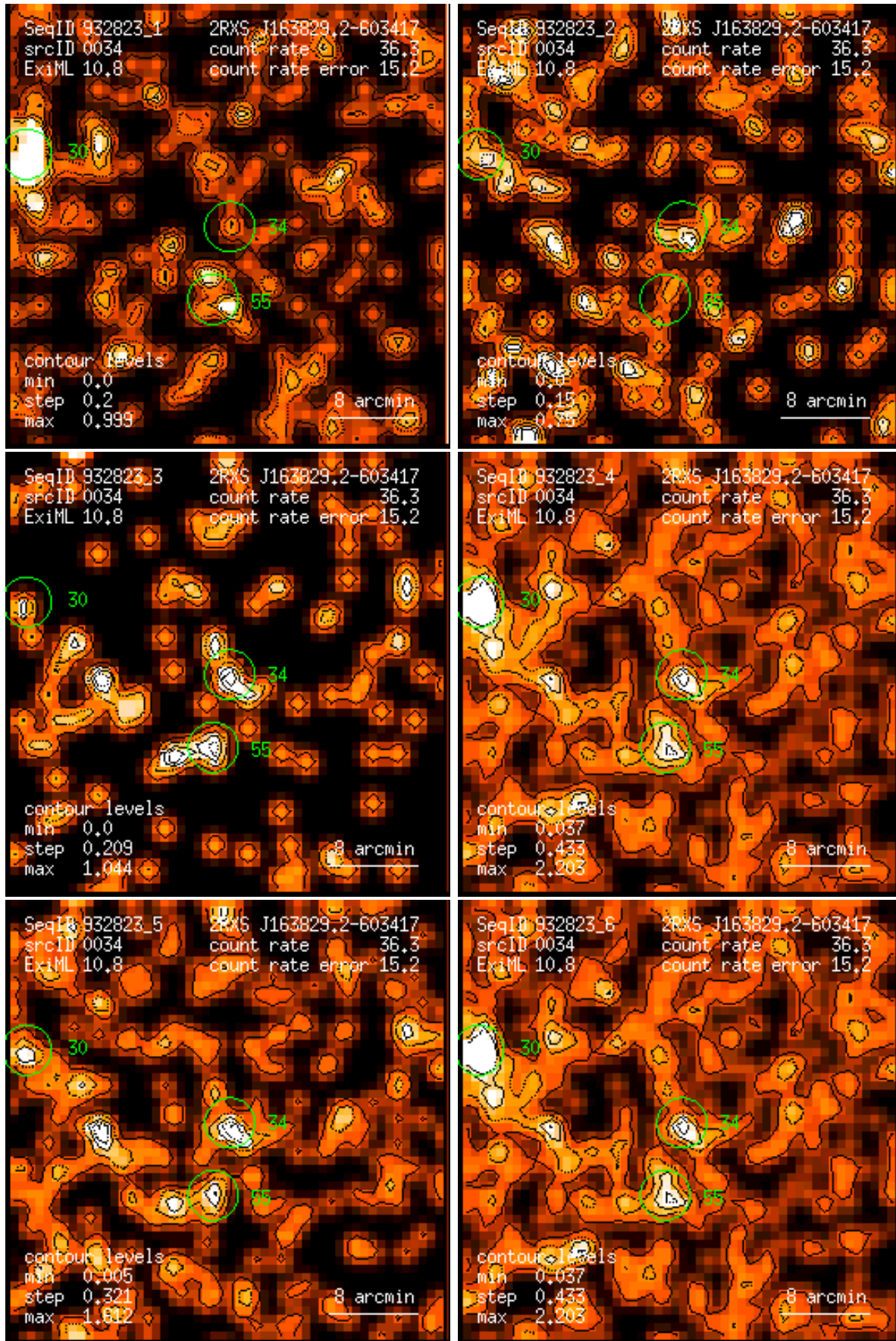
Figure 34: RASS 932823: detection 0034: band rate images, Gaussian filter: (1) PSPC channels 11 – 41, (2) 52 – 90, (3) 91 – 201, (4) 11 – 235, (5) 52 – 201, (6) 11 – 201. Broad band rates in counts/ks. Band rate contour levels in counts/ks/arcmin 2 .
