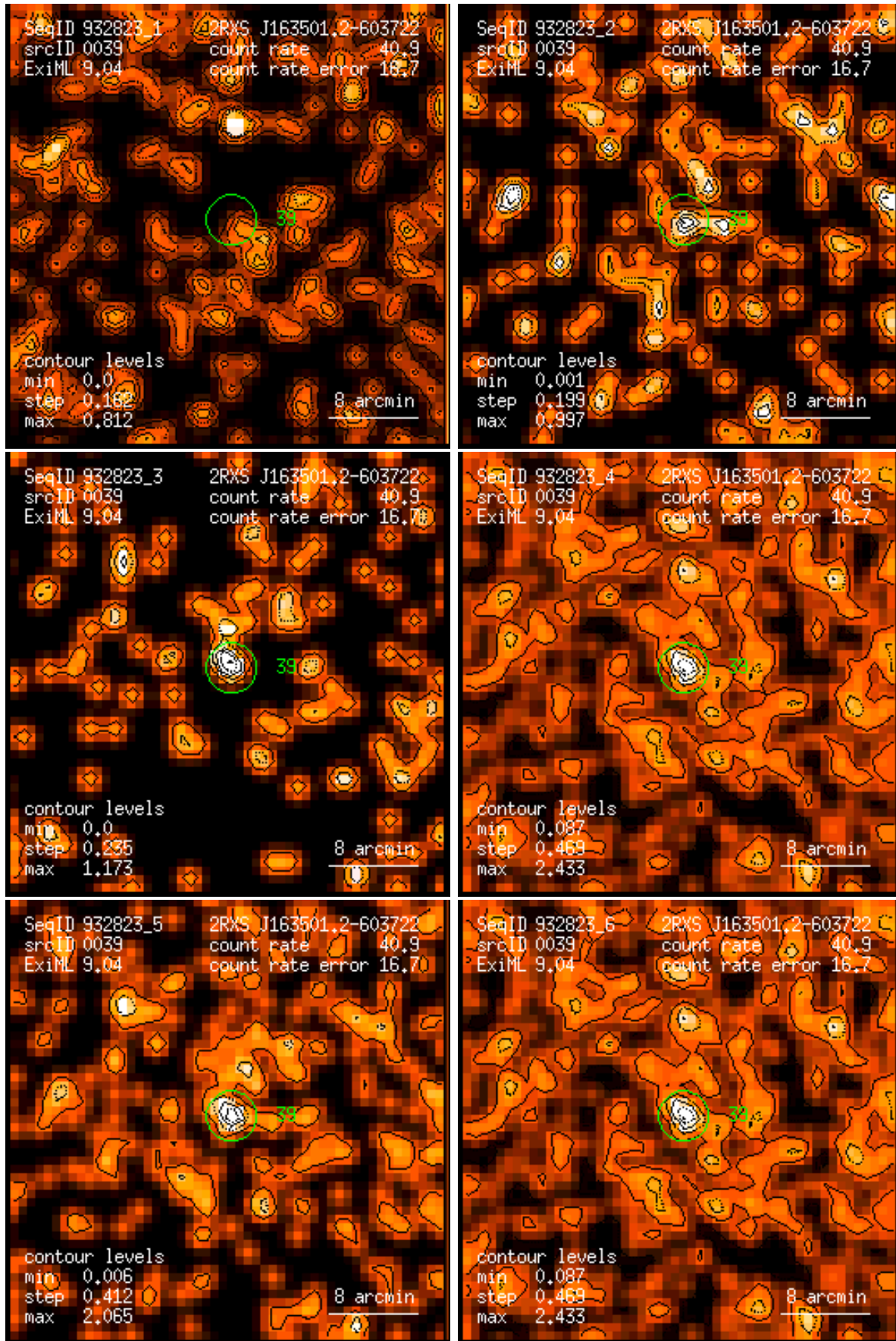
Figure 39: RASS 932823: detection 0039: band rate images, Gaussian filter: (1) PSPC channels 11 – 41, (2) 52 – 90, (3) 91 – 201, (4) 11 – 235, (5) 52 – 201, (6) 11 – 201. Broad band rates in counts/ks. Band rate contour levels in counts/ks/arcmin 2 .
