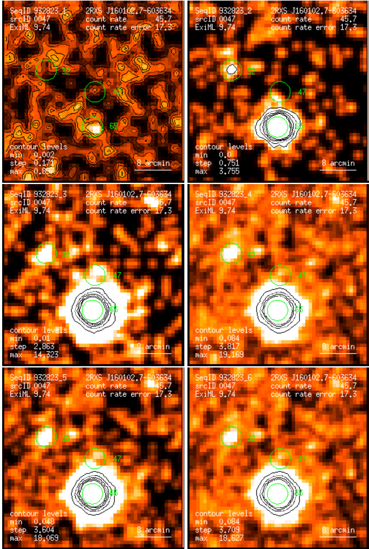
Figure 47: RASS 932823: detection 0047: band rate images, Gaussian filter: (1) PSPC channels 11 – 41, (2) 52 – 90, (3) 91 – 201, (4) 11 – 235, (5) 52 – 201, (6) 11 – 201. Broad band rates in counts/ks. Band rate contour levels in counts/ks/arcmin 2 .
