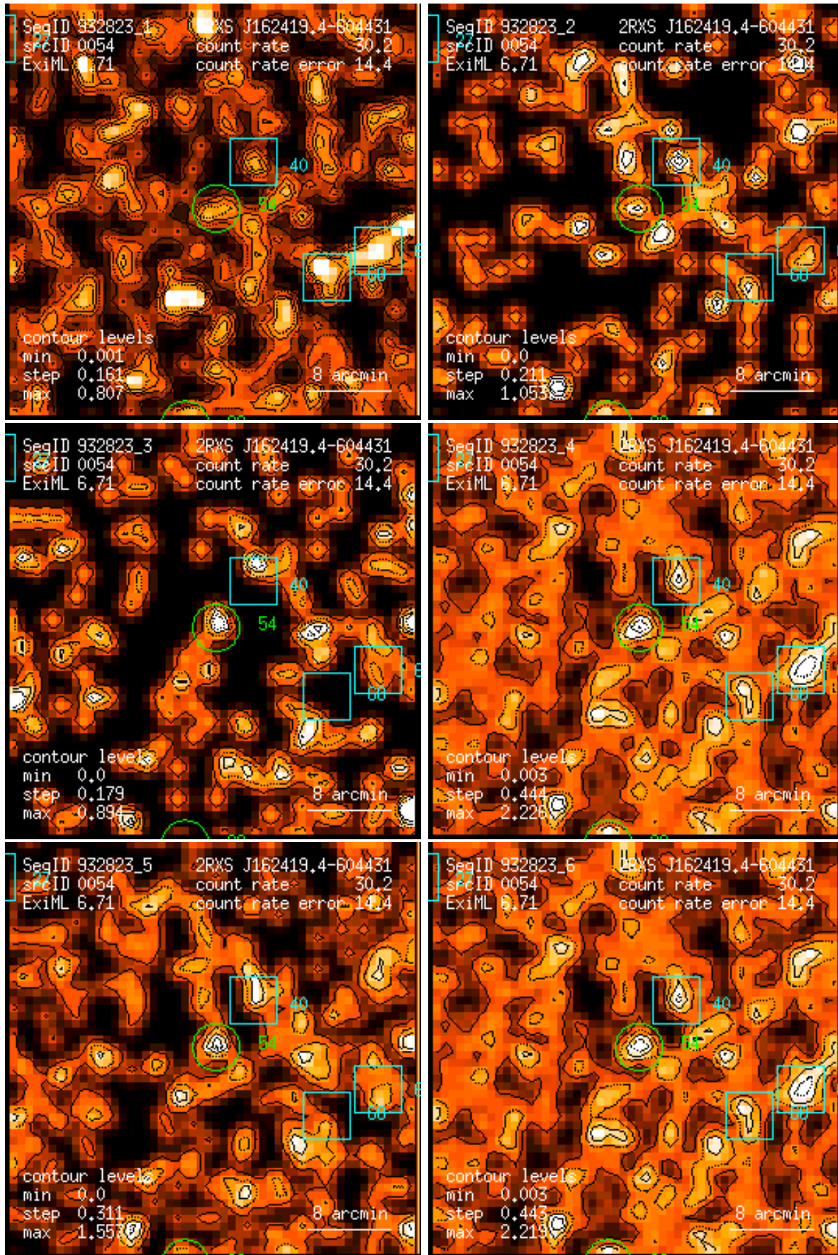
Figure 54: RASS 932823: detection 0054: band rate images, Gaussian filter: (1) PSPC channels 11 – 41, (2) 52 – 90, (3) 91 – 201, (4) 11 – 235, (5) 52 – 201, (6) 11 – 201. Broad band rates in counts/ks. Band rate contour levels in counts/ks/arcmin 2 .
