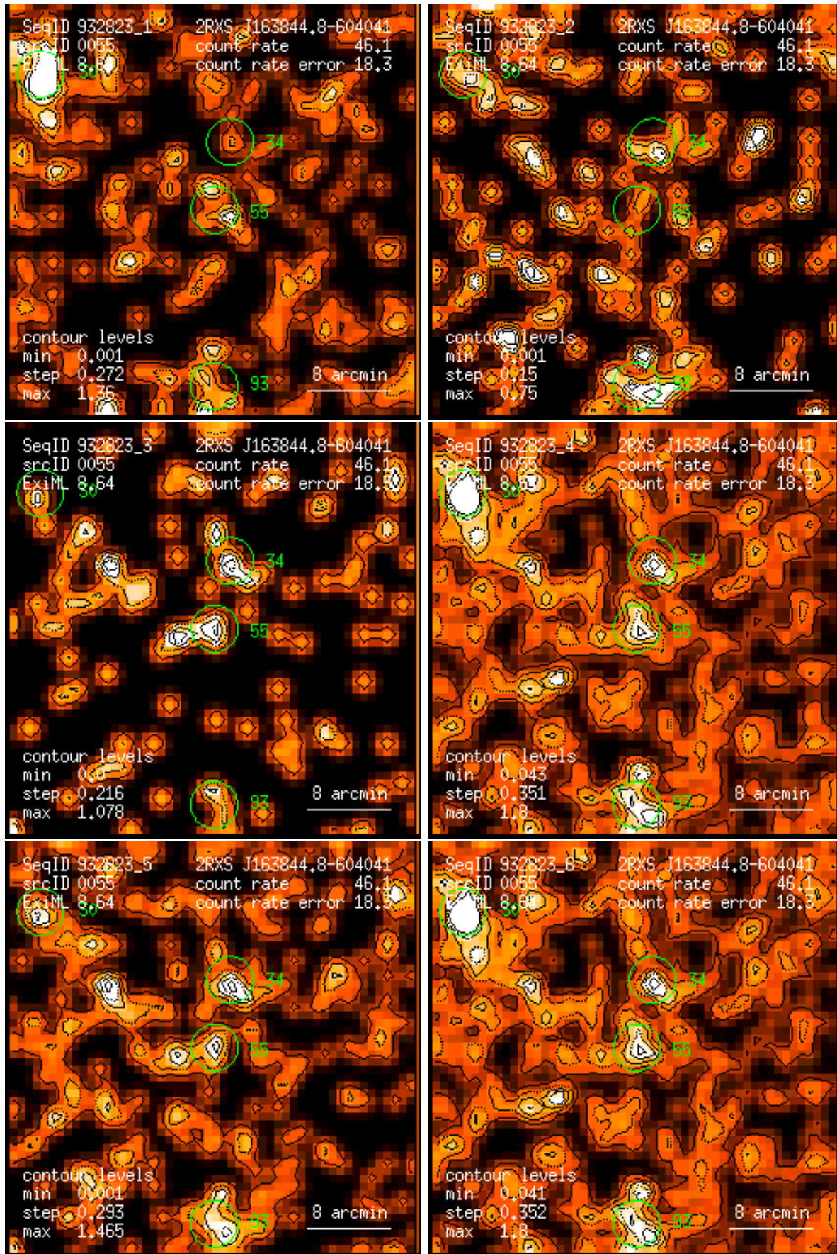
Figure 55: RASS 932823: detection 0055: band rate images, Gaussian filter: (1) PSPC channels 11 – 41, (2) 52 – 90, (3) 91 – 201, (4) 11 – 235, (5) 52 – 201, (6) 11 – 201. Broad band rates in counts/ks. Band rate contour levels in counts/ks/arcmin 2 .
