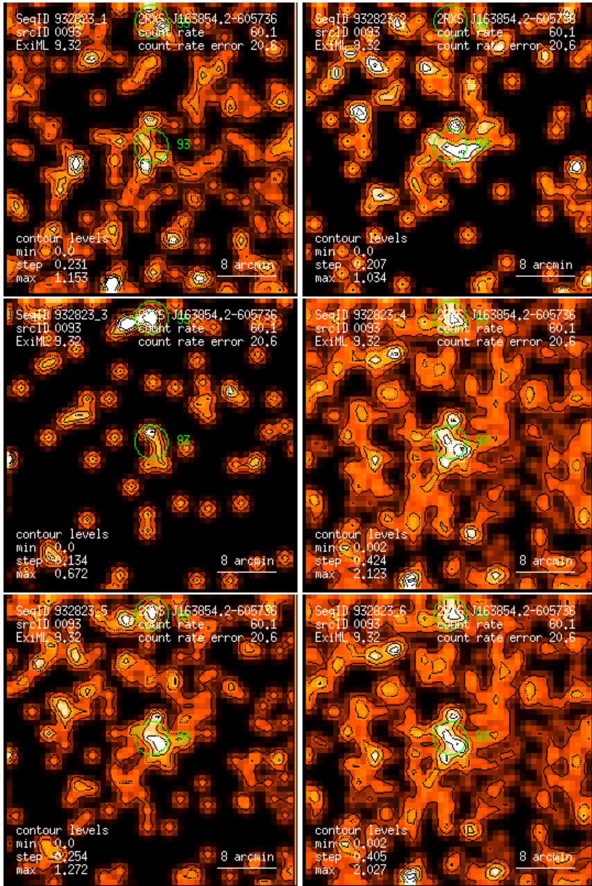
Figure 93: RASS 932823: detection 0093: band rate images, Gaussian filter: (1) PSPC channels 11 – 41, (2) 52 – 90, (3) 91 – 201, (4) 11 – 235, (5) 52 – 201, (6) 11 – 201. Broad band rates in counts/ks. Band rate contour levels in counts/ks/arcmin 2 .
