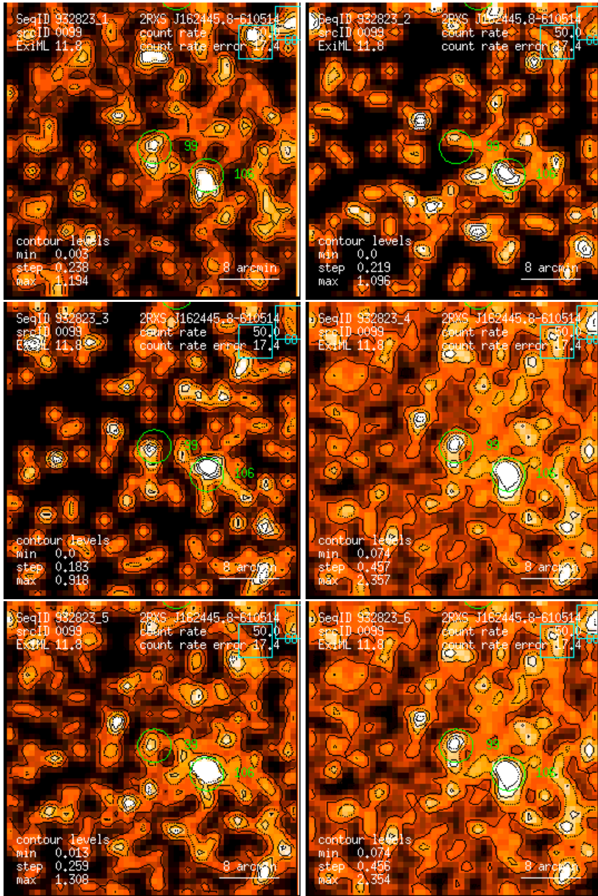
Figure 99: RASS 932823: detection 0099: band rate images, Gaussian filter: (1) PSPC channels 11 – 41, (2) 52 – 90, (3) 91 – 201, (4) 11 – 235, (5) 52 – 201, (6) 11 – 201. Broad band rates in counts/ks. Band rate contour levels in counts/ks/arcmin 2 .
