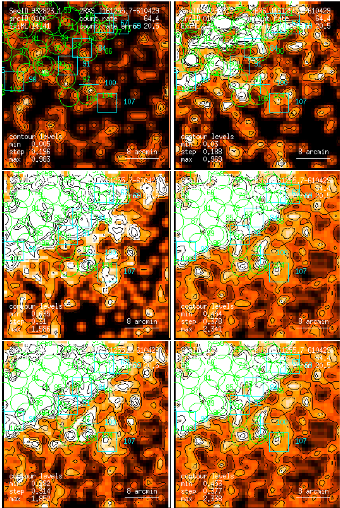
Figure 100: RASS 932823: detection 0100: band rate images, Gaussian filter: (1) PSPC channels 11 – 41, (2) 52 – 90, (3) 91 – 201, (4) 11 – 235, (5) 52 – 201, (6) 11 – 201. Broad band rates in counts/ks. Band rate contour levels in counts/ks/arcmin 2 .
