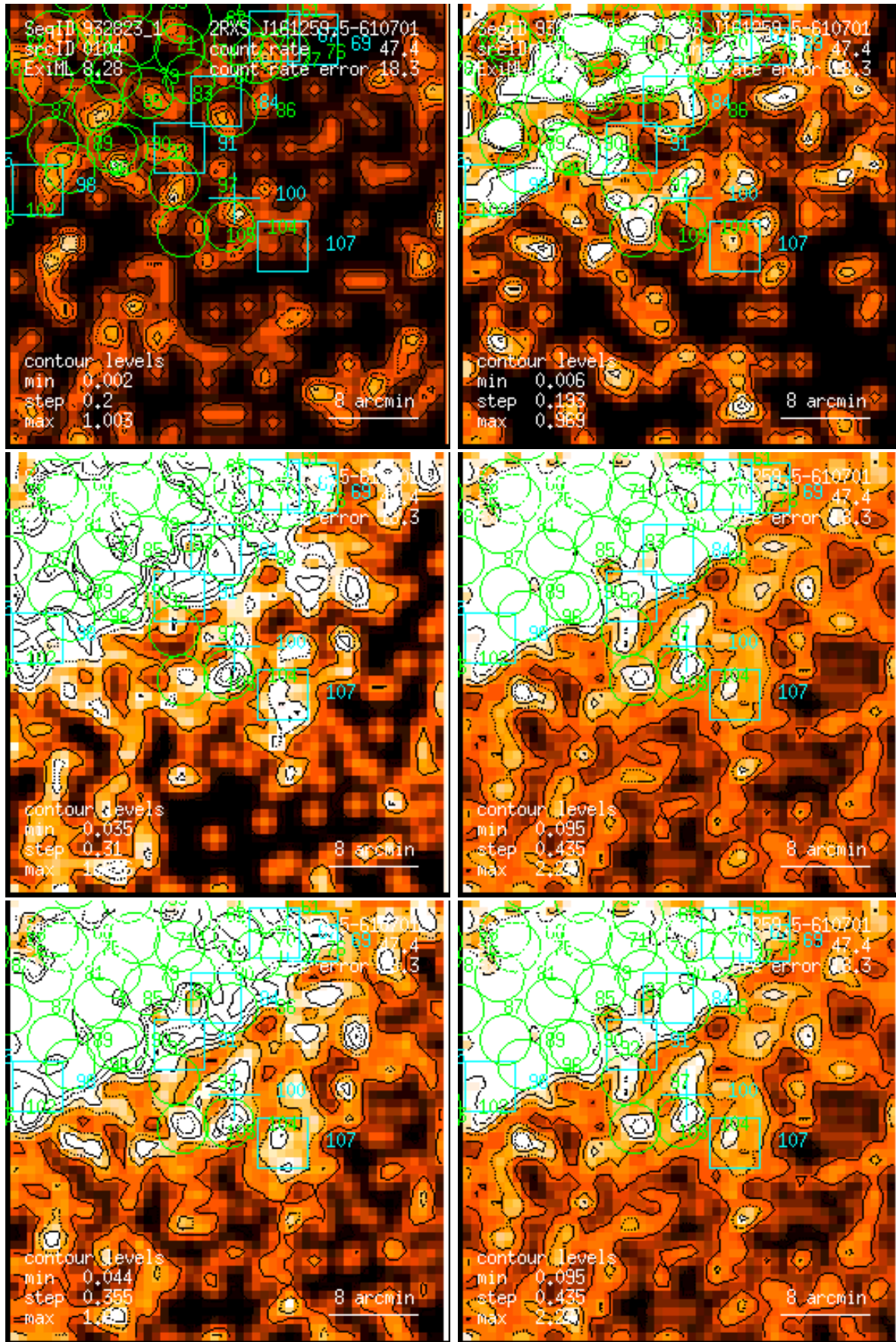
Figure 104: RASS 932823: detection 0104: band rate images, Gaussian filter: (1) PSPC channels 11 – 41, (2) 52 – 90, (3) 91 – 201, (4) 11 – 235, (5) 52 – 201, (6) 11 – 201. Broad band rates in counts/ks. Band rate contour levels in counts/ks/arcmin 2 .
