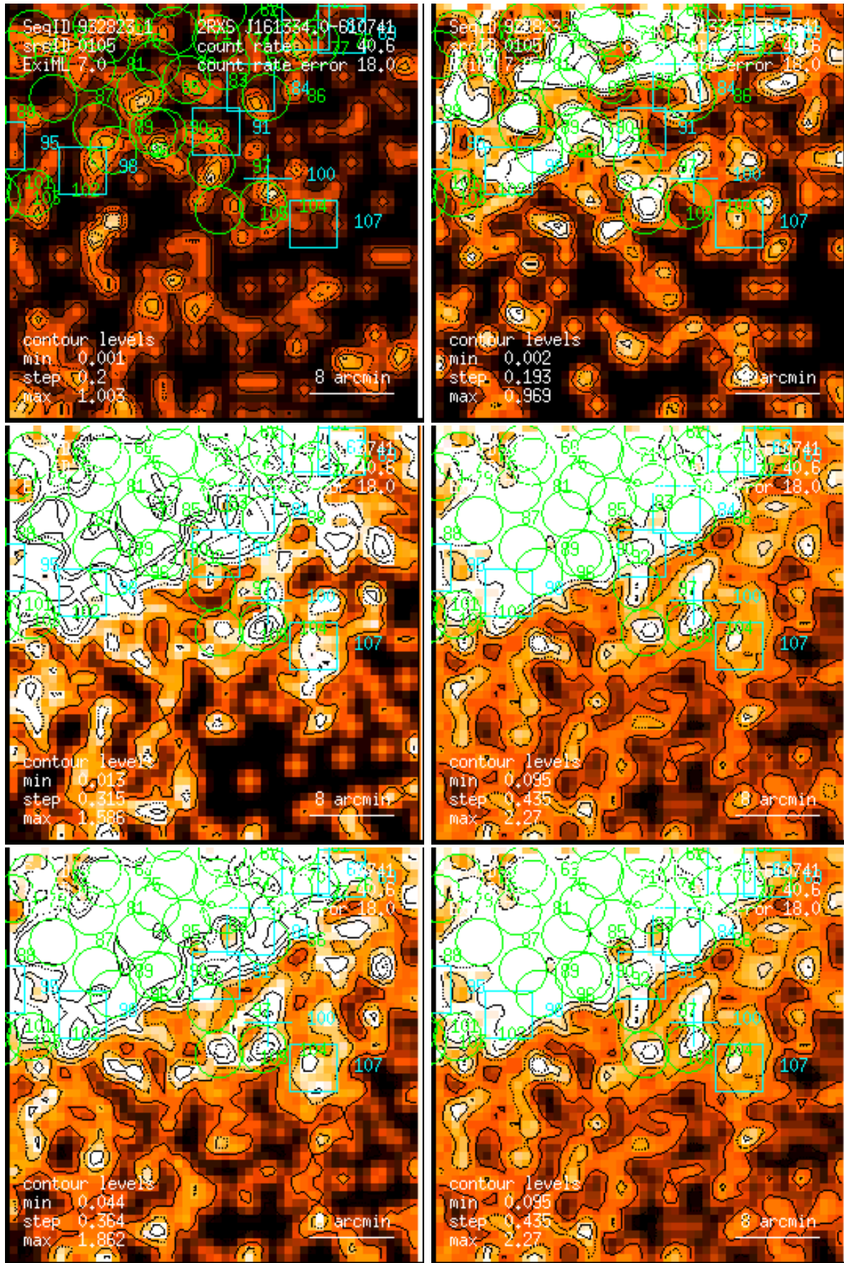
Figure 105: RASS 932823: detection 0105: band rate images, Gaussian filter: (1) PSPC channels 11 – 41, (2) 52 – 90, (3) 91 – 201, (4) 11 – 235, (5) 52 – 201, (6) 11 – 201. Broad band rates in counts/ks. Band rate contour levels in counts/ks/arcmin 2 .
