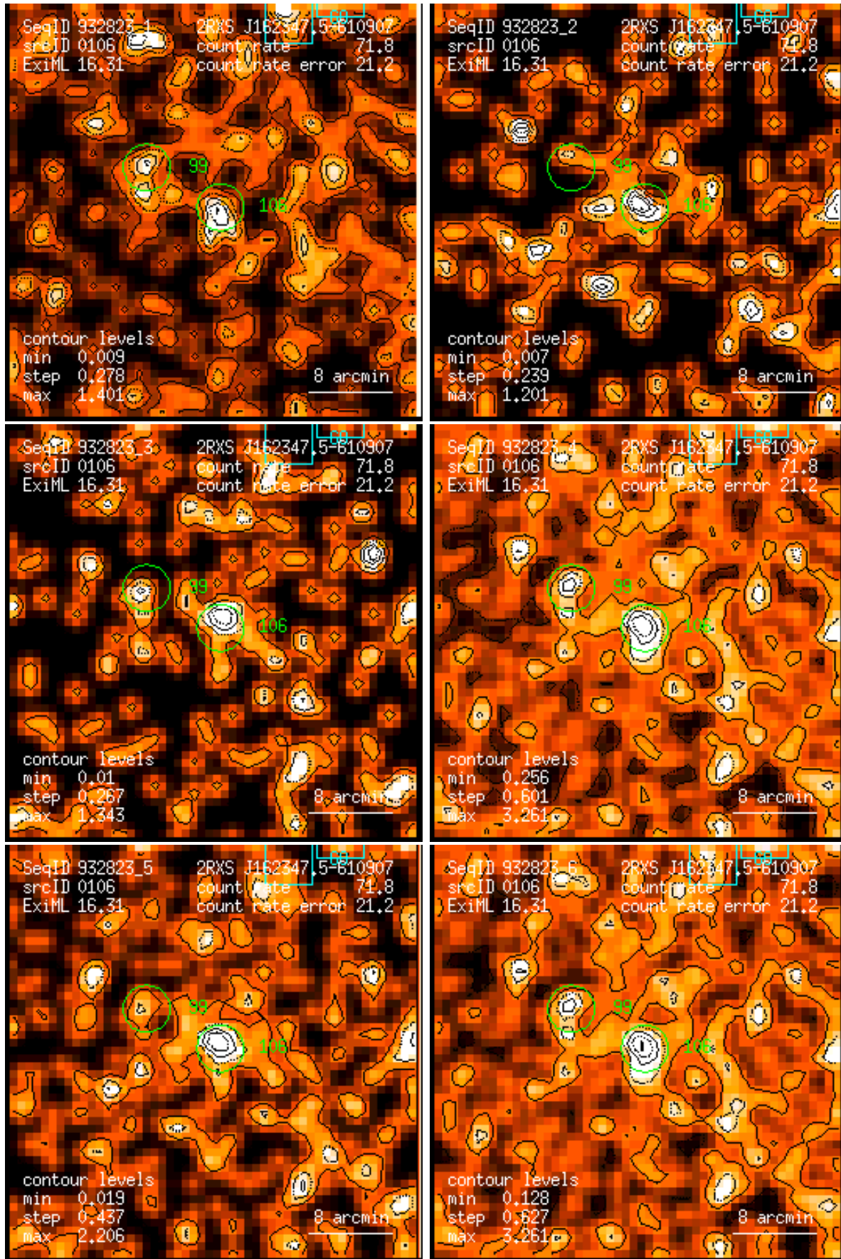
Figure 106: RASS 932823: detection 0106: band rate images, Gaussian filter: (1) PSPC channels 11 – 41, (2) 52 – 90, (3) 91 – 201, (4) 11 – 235, (5) 52 – 201, (6) 11 – 201. Broad band rates in counts/ks. Band rate contour levels in counts/ks/arcmin 2 .
