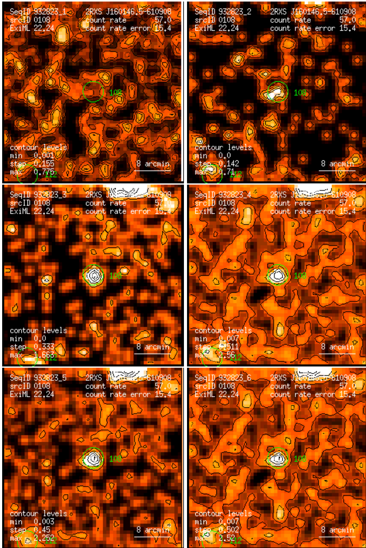
Figure 108: RASS 932823: detection 0108: band rate images, Gaussian filter: (1) PSPC channels 11 – 41, (2) 52 – 90, (3) 91 – 201, (4) 11 – 235, (5) 52 – 201, (6) 11 – 201. Broad band rates in counts/ks. Band rate contour levels in counts/ks/arcmin 2 .
