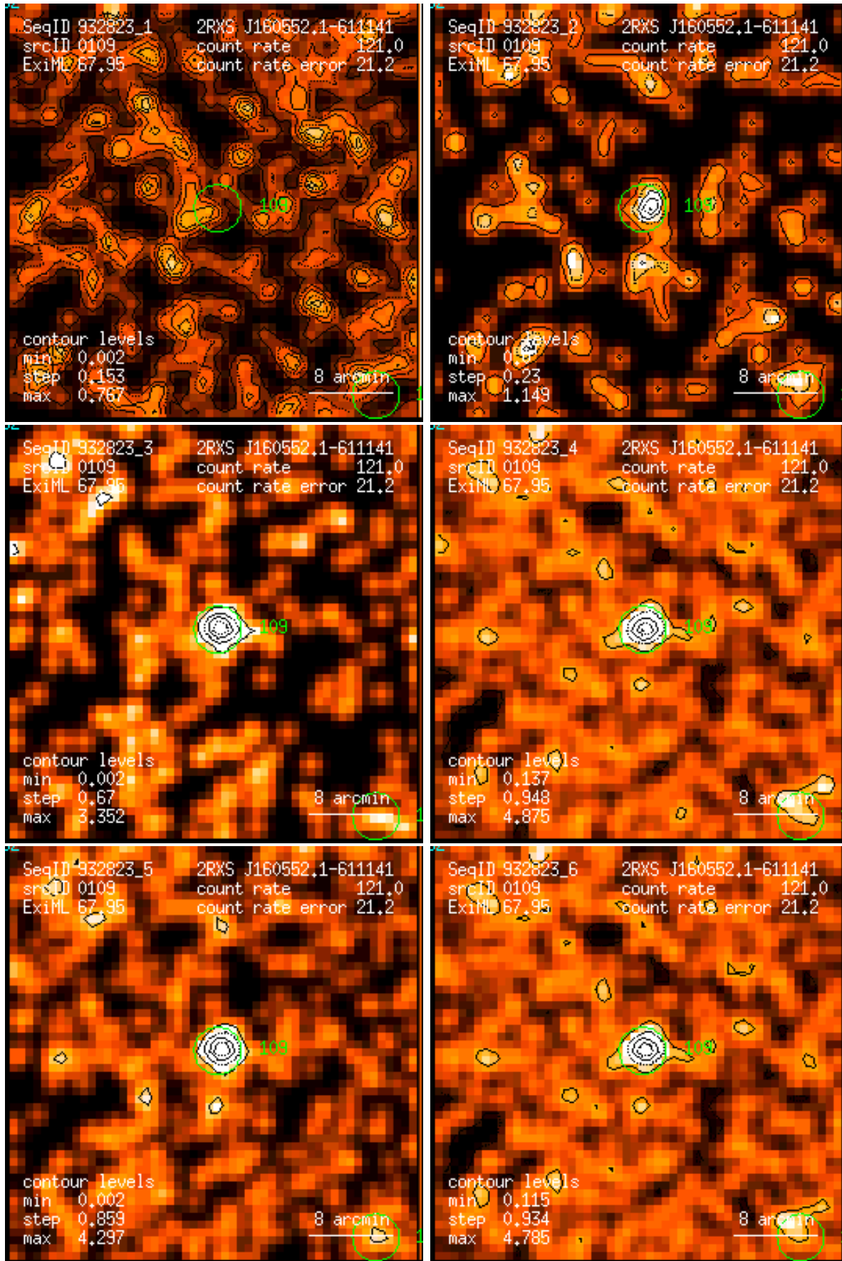
Figure 109: RASS 932823: detection 0109: band rate images, Gaussian filter: (1) PSPC channels 11 – 41, (2) 52 – 90, (3) 91 – 201, (4) 11 – 235, (5) 52 – 201, (6) 11 – 201. Broad band rates in counts/ks. Band rate contour levels in counts/ks/arcmin 2 .
