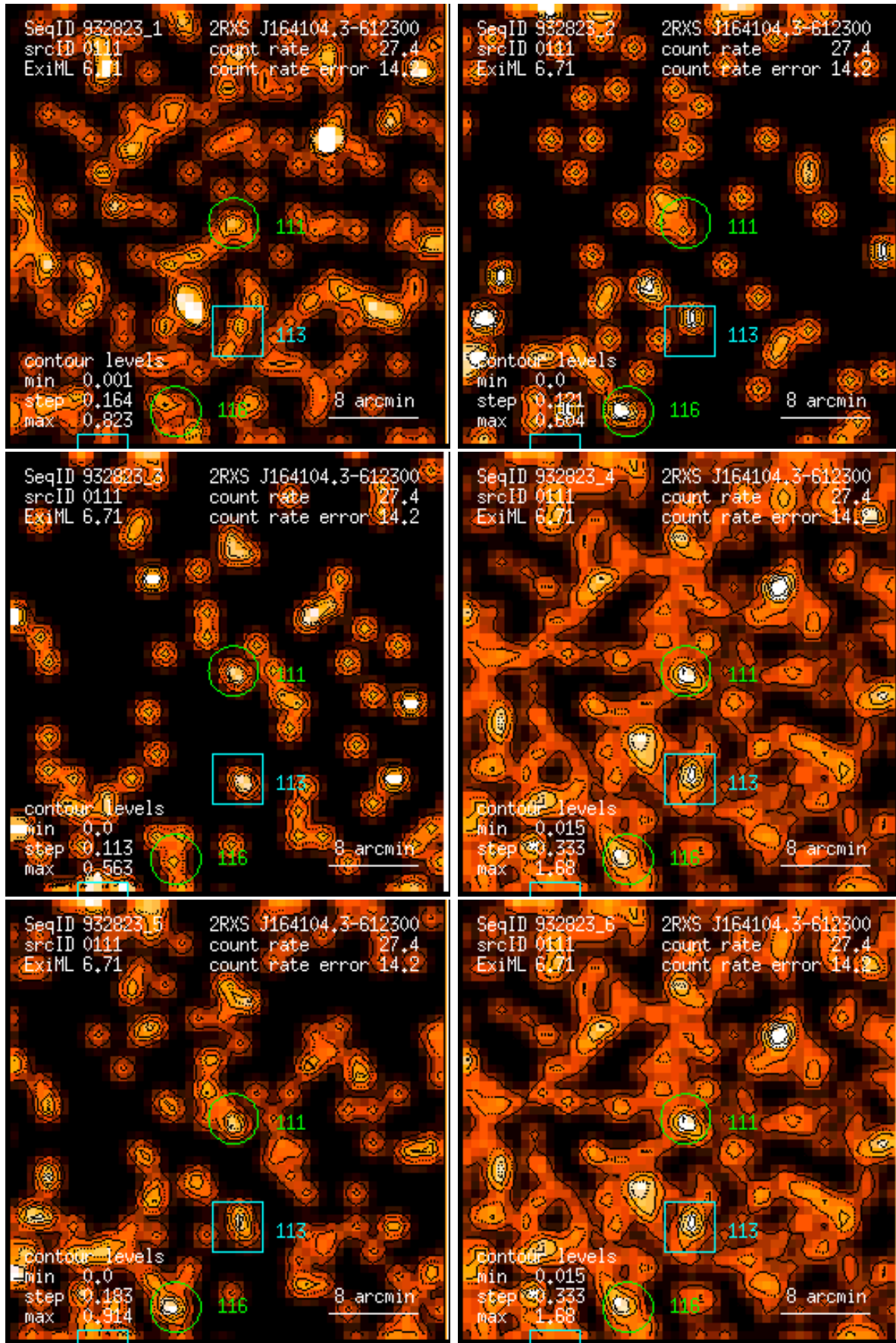
Figure 111: RASS 932823: detection 0111: band rate images, Gaussian filter: (1) PSPC channels 11 – 41, (2) 52 – 90, (3) 91 – 201, (4) 11 – 235, (5) 52 – 201, (6) 11 – 201. Broad band rates in counts/ks. Band rate contour levels in counts/ks/arcmin 2 .
