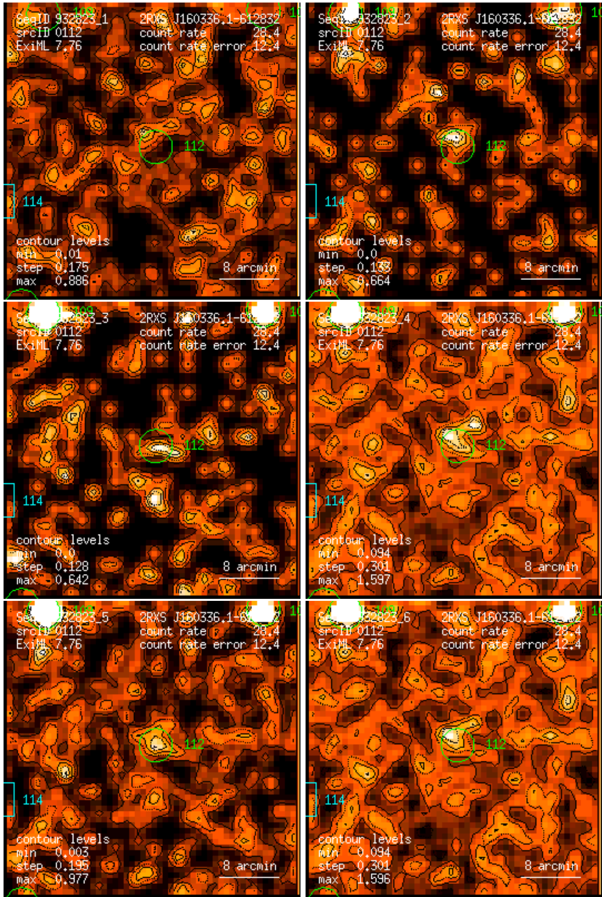
Figure 112: RASS 932823: detection 0112: band rate images, Gaussian filter: (1) PSPC channels 11 – 41, (2) 52 – 90, (3) 91 – 201, (4) 11 – 235, (5) 52 – 201, (6) 11 – 201. Broad band rates in counts/ks. Band rate contour levels in counts/ks/arcmin 2 .
