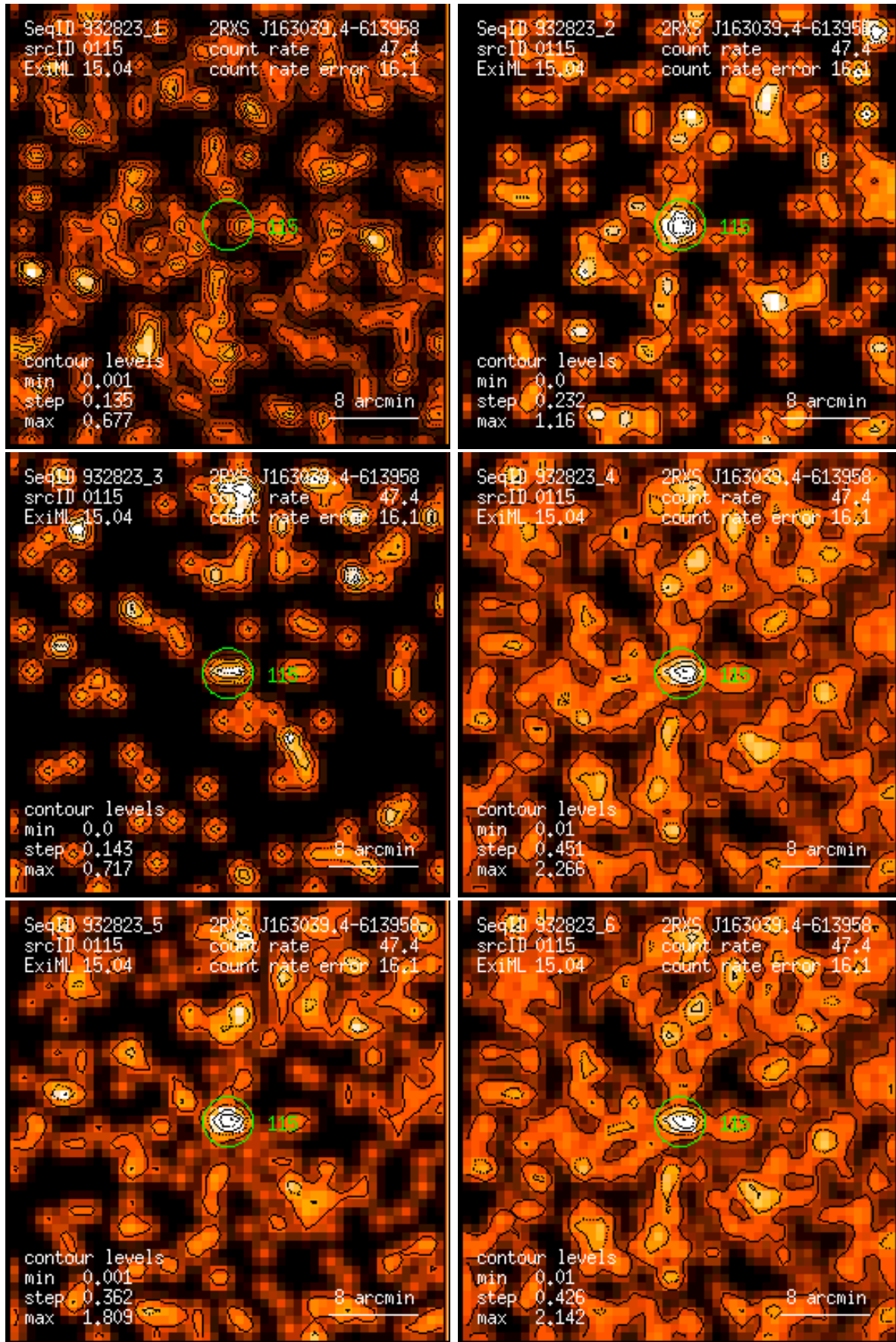
Figure 115: RASS 932823: detection 0115: band rate images, Gaussian filter: (1) PSPC channels 11 – 41, (2) 52 – 90, (3) 91 – 201, (4) 11 – 235, (5) 52 – 201, (6) 11 – 201. Broad band rates in counts/ks. Band rate contour levels in counts/ks/arcmin 2 .
