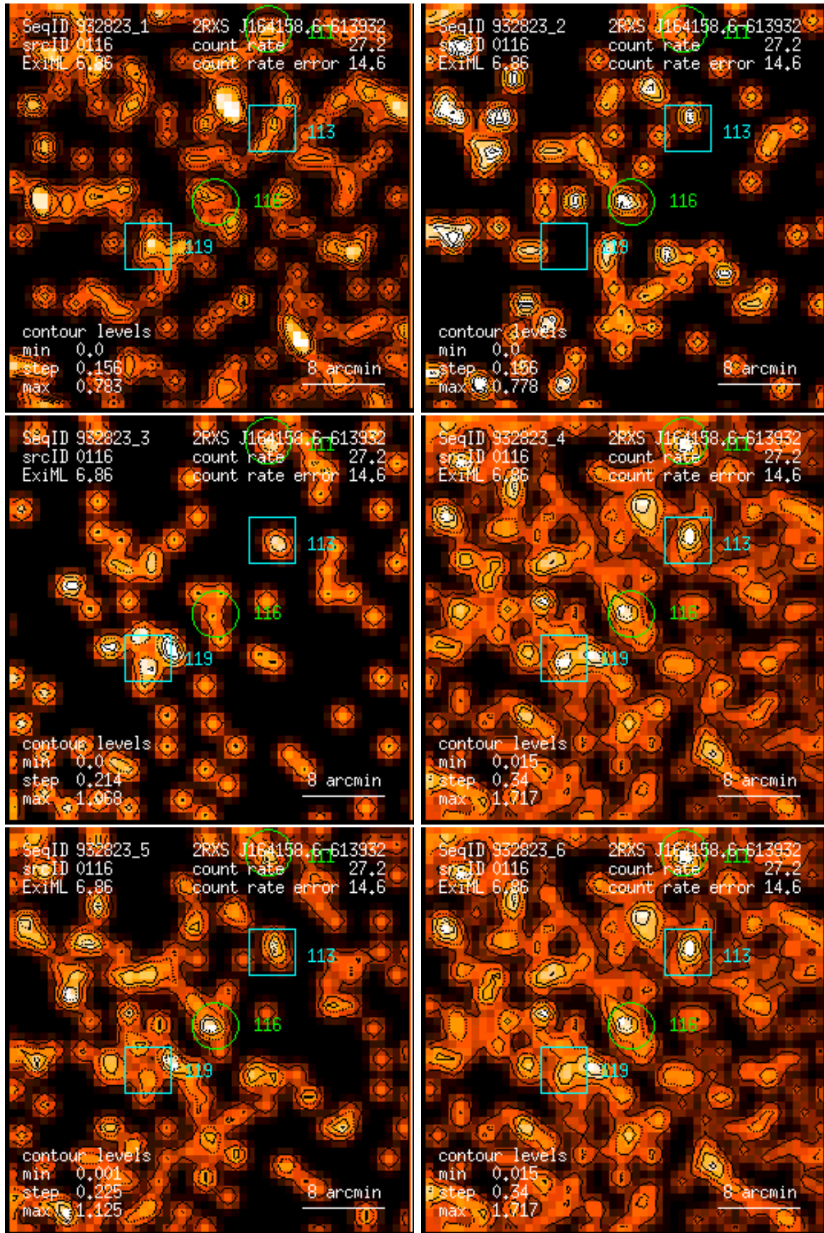
Figure 116: RASS 932823: detection 0116: band rate images, Gaussian filter: (1) PSPC channels 11 – 41, (2) 52 – 90, (3) 91 – 201, (4) 11 – 235, (5) 52 – 201, (6) 11 – 201. Broad band rates in counts/ks. Band rate contour levels in counts/ks/arcmin 2 .
