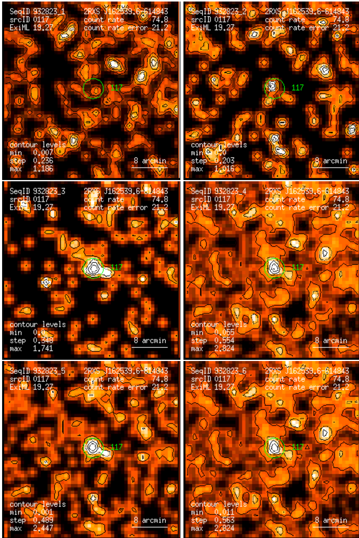
Figure 117: RASS 932823: detection 0117: band rate images, Gaussian filter: (1) PSPC channels 11 – 41, (2) 52 – 90, (3) 91 – 201, (4) 11 – 235, (5) 52 – 201, (6) 11 – 201. Broad band rates in counts/ks. Band rate contour levels in counts/ks/arcmin 2 .
